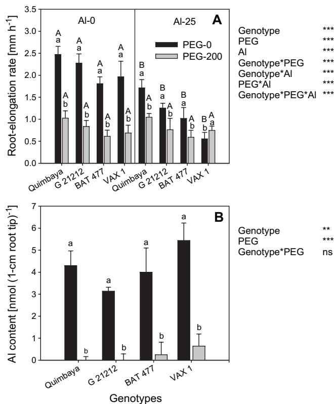
Fig. 1. Root elongation rate (A) and Al content of 1 cm root tips (B) of four common bean genotypes under osmotic (200 g l -1 PEG) and Al stress (25 \mu M Al). Plants were pre-cultured in a simplified nutrient solution containing 5 mM CaCl 2 , 1 mM KCl, and 8 \mu M H 3 BO 3 for 48 h for acclimation and pH adaptation, then treated without or with 25 \mu M Al in the absence or presence of 200 g l -1 PEG in the simplified nutrient solution for 24 h, pH 4.5. Bars represent means \pm SD, n =12 for (A) and n =4 for (B). Means with the same small letter and capital letter are not significantly different at P < 0.05 ( t test) for the comparison of PEG treatments within Al supplies and comparison of Al treatments within PEG supplies, respectively. For the ANOVA, **, *** denote significant differences at P < 0.01, P < 0.001, respectively; ns, not significant.
