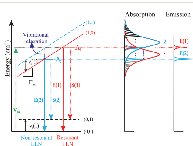
Fig. 1 Energy-level diagram illustrating resonant LLN E(1) and non-resonant LLN E(2) after site-selective laser excitation at an energy, \nu_{\text{ex}} (diagram adapted from Jankowiak 35 ). See text for a detailed explanation.
