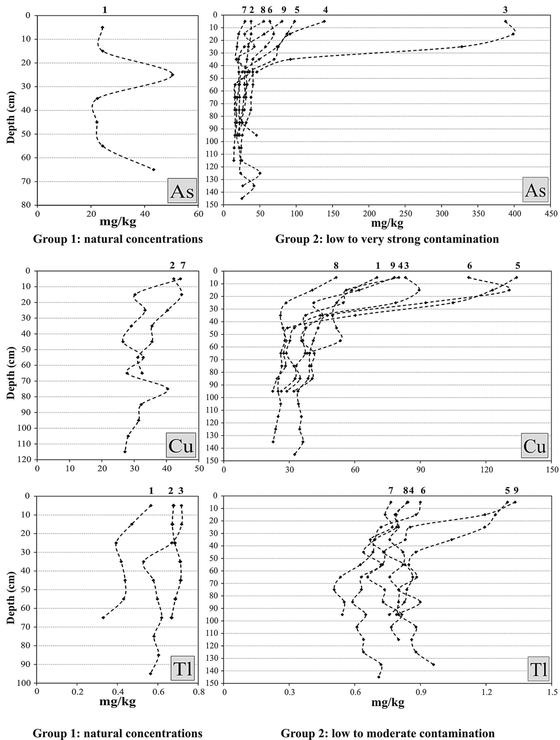
Fig. 3 Vertical distribution of As, Cu and Tl concentrations in soil profiles (soil profile identification is at the top of each graph)
