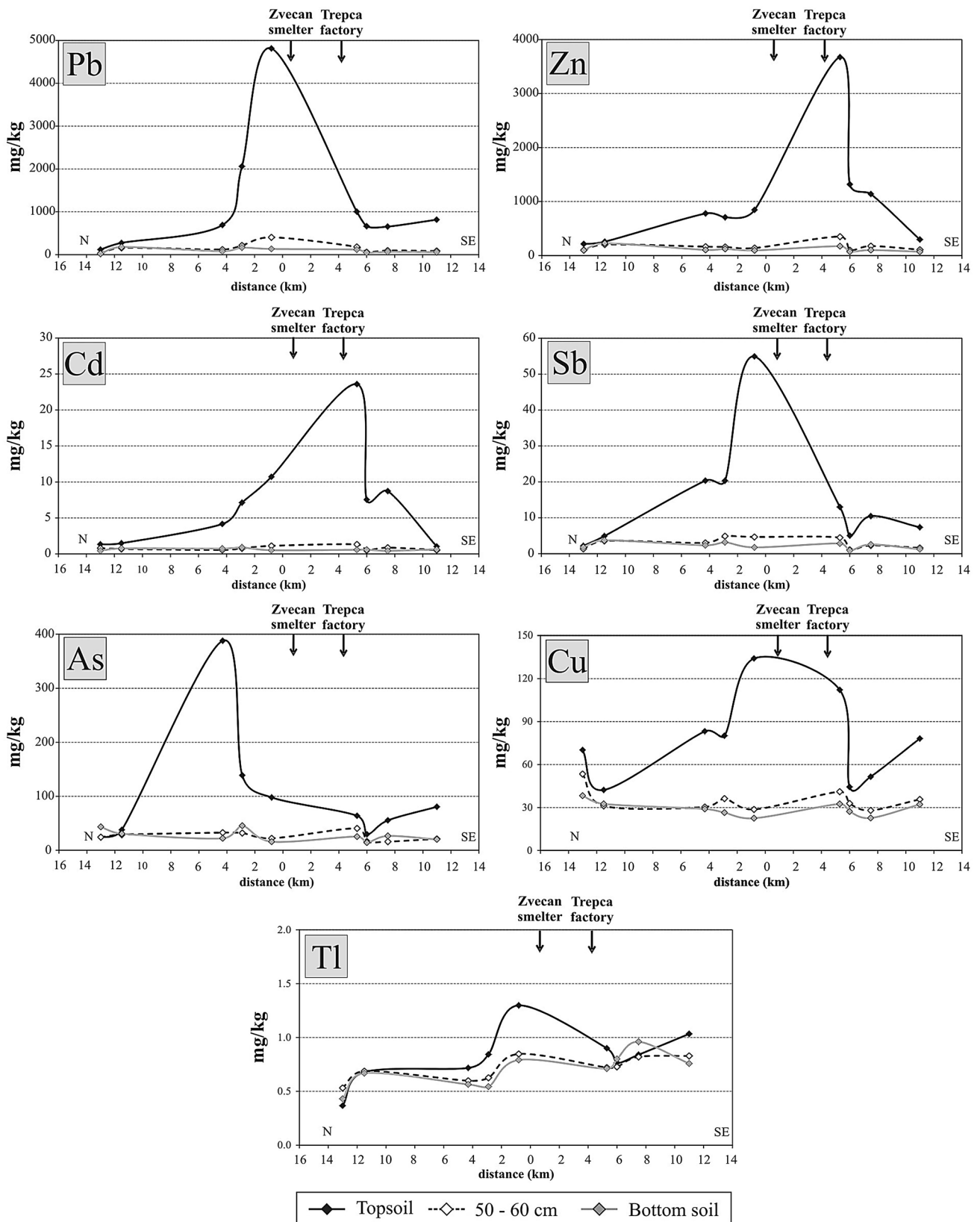
Fig. 4 Surface and vertical distribution of As, Cd, Cu, Pb, Sb, Tl and Zn concentrations in relation to distance from the Zvecan smelter along the transects N and SE
