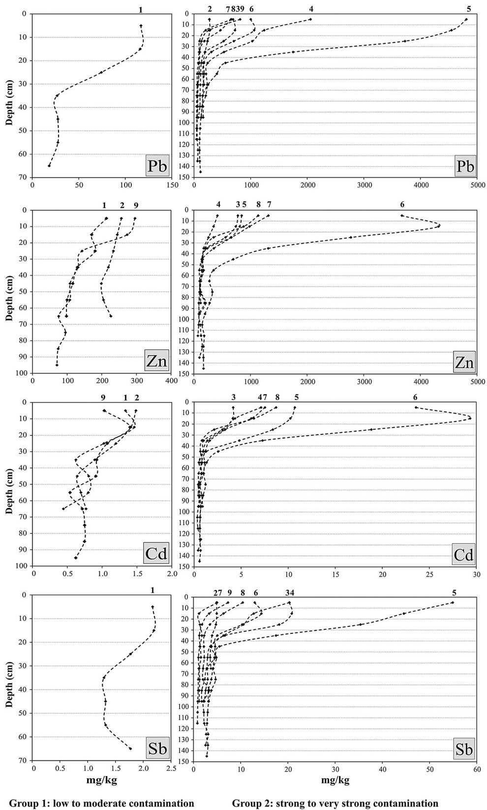
Fig. 2 Vertical distribution of Cd, Pb, Sb and Zn concentrations in soil profiles (soil profile identification is at the top of each graph)
