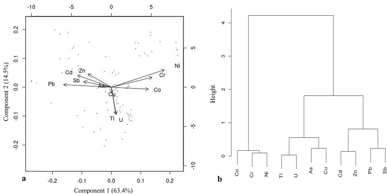
Fig. 5 Grouping of the potentially toxic elements (PTEs) by compositional multivariate statistical analysis: a principal component analysis (PCA) biplot; b Q-mode cluster analysis (CA) dendrogram
