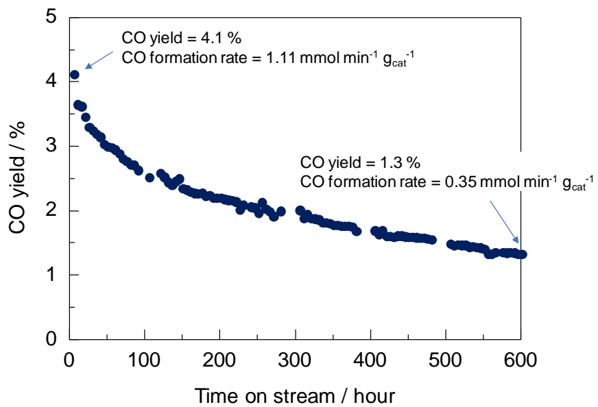
Figure 6. Long-term stability test for the RWGS reaction over Pt(3)/MoO x (15)/TiO 2 . Reaction conditions: catalyst (15 mg), CO 2 :H 2 :He:N 2 = 10:40:45:5, 100 mL min -1 , 250 °C.
