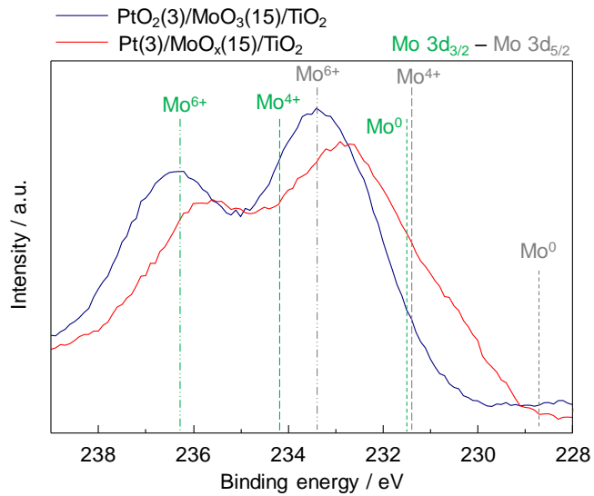
Figure 2. XPS spectra of the Mo 3d region of PtO 2 (3)/MoO 3 (15)/TiO 2 (unreduced sample; navy) and Pt(3)/MoO x (15)/TiO 2 (reduced sample; red).
