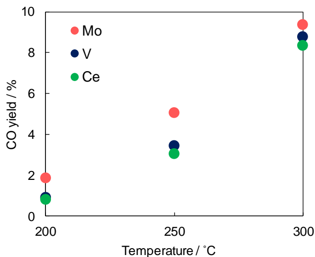
Figure 3. RWGS reaction over Pt(3)/MoO x (15)/TiO 2 , Pt(3)/VO x /TiO 2 , and Pt(3)/CeO x /TiO 2 . Catalyst (15 mg), CO 2 :H 2 :He:N 2 = 10:40:45:5, 100 mL min -1 .
