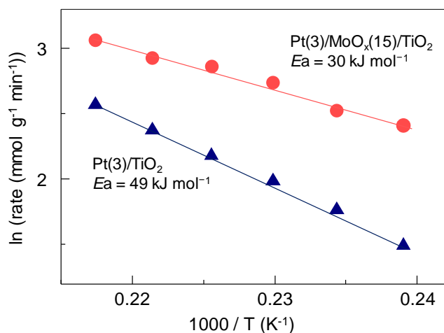
Figure 5. Arrhenius plot for the RWGS reaction over Pt(3)/MoO x (15)/TiO 2 and Pt(3)/TiO 2 . Catalyst (5 mg), CO 2 :H 2 :He:N 2 = 10:40:45:5, 100 mL min -1 , 230-280 °C.
