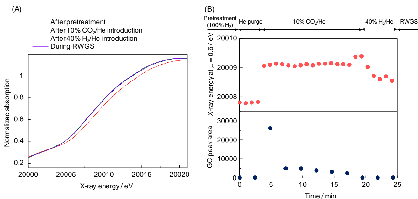
Figure 7. (A) Operando Mo K-edge XANES of Pt(3)/MoO x (15)/TiO 2 obtained at 250 °C after the H 2 reduction pretreatment (navy blue line) and after subsequent introduction of 10%CO 2 /He (red line). (B) Results of the operando Mo K-edge XAS measurements. Changes in the shift of the absorption edge and the amount of CO in the gas phase (GC peak area) under flowing 10%CO 2 /He, 40%H 2 /He, and 10%CO 2 +40%H 2 /He at 250 °C.
