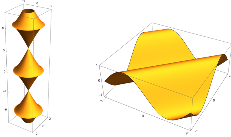
FIGURE 2. Left: an indefinite improper affine map f , which is a series of surfaces in Figure 1, joined along cuspidal edges and at cone points. Right: the graph of \omega , which gives the affine metric of f apart from S .
