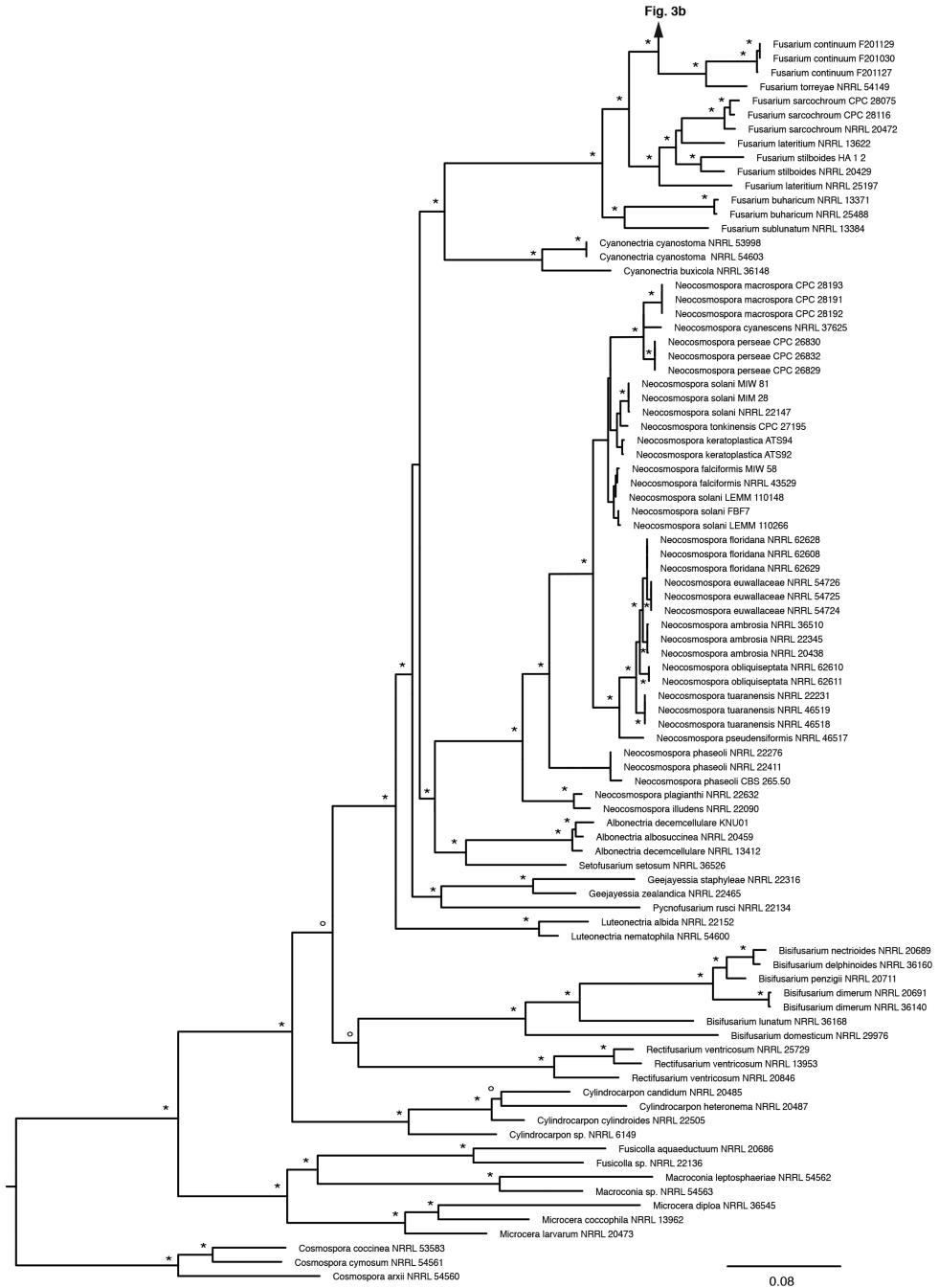
Figure 3. Maximum Likelihood topology obtained via heuristic search algorithm of the combined rpb1 , rpb2 and tefla data matrix. Bootstrap support (ML-BS) values above 50 are indicated with a dot, ML-BS values above 75 are indicated with an asterisk. No indication above the branches indicates a ML-BS value below 50. Newly included accessions are indicated in red. FOSC: Fusarium oxysporum species complex, FFSC: Fusarium fujikuroi species complex.
