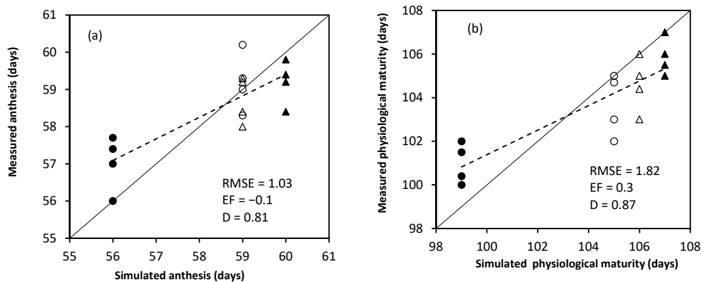
Figure 4. Comparison of simulated and measured anthesis (a), physiological maturity (b), grain yield at maturity (c) and shoot dry matter at maturity (d) for SAMMAZ-15 using Iburu and Zaria experimental data sets. (Iburu = ▲2015, ○2016 and Zaria = ●2015, △2016, the plants were grown under four N treatments within each location and date).
