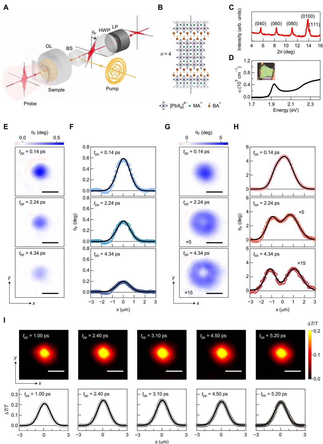
Fig. 1. Time-resolved Faraday rotation imaging of spin-polarized excitons in 2D RPP (BA) 2 (MA) 3 Pb 4 I 13 . (A) Illustration of the time-resolved Faraday rotation imaging setup. OL, objective lens; BS, beam splitter; HWP, half-wave plate; LP, linear polarizer. (B) Schematic crystal structure of 2D RPP (BA) 2 (MA) 3 Pb 4 I 13 ( n = 4 ). (C) X-ray diffraction spectrum of (BA) 2 (MA) 3 Pb 4 I 13 crystals. The vertical axis is in log scale. (D) Absorption coefficient spectrum of an exfoliated sample. The inset is an optical microscope image of the sample. Scale bar, 10 \mu\text{m} . (E) Images of pump-induced Faraday rotation angle at pump-probe delay times of 0.14, 2.24, and 4.34 ps for an exciton density per 2D perovskite layer of 6.8 \times 10^{11} \text{ cm}^{-2} . Scale bars, 2 \mu\text{m} . (F) Spatial profiles of pump-induced Faraday rotation angle, which correspond to the horizontal cross sections of the images in (E) passing through the center of the excitation spot ( x = y = 0 \mu\text{m} ). The black curves are Gaussian fits. (G and H) Same as (E) and (F) but for an exciton density per 2D perovskite layer of 1.2 \times 10^{13} \text{ cm}^{-2} . The middle and bottom panels of (G) and (H) are magnified by factors of 5 and 15, respectively. The black curves in (H) are double-Gaussian fits. (I) Top: Time-resolved images of pump-induced change in transmission at various pump-probe delay times for n_{\text{ex}} = 1.3 \times 10^{13} \text{ cm}^{-2} . Scale bars, 2 \mu\text{m} . Bottom: Spatial profiles of pump-induced change in transmission, which correspond to the horizontal cross sections of the images shown in the top panels passing through the center of the excitation spot ( x = y = 0 \mu\text{m} ). The black curves are Gaussian fits.
