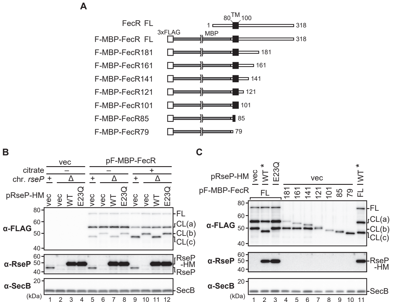
Figure 4. RseP cleaves the transmembrane region of FecR. A , schematic representations of FecR, the F-MBP-FecR model substrate, and the truncated derivatives of F-MBP-FecR. The regions corresponding to the FecR-derived cytoplasmic and periplasmic domains are shown as white lines , MBP as the gray line , the predicted transmembrane region as a black box , and 3xFLAG tag as a white box , respectively. B , behavior of the F-MBP-FecR protein in response to the co-expression of RseP and the addition of Na 3 -citrate. YK167 ( \Delta rseA , rseP + ) or YK191 ( \Delta rseA \Delta rseP ) cells harboring pTWV228 (vec) or pYK147 (pF-MBP-FecR) were further transformed with pSTD689 (vec), pYH9 (RseP-HM, WT), or pYH13 (RseP(E23Q)-HM, E23Q). The cells were grown as in Figure 3C. The proteins were analyzed by 10% Laemmli SDS-PAGE and anti-FLAG immunoblotting or 12.5% Laemmli SDS-PAGE and anti-RseP ( \alpha -RseP), or anti-SecB ( \alpha -SecB) immunoblotting. The band intensity of RseP-HM is saturated. C , behaviors of the truncated derivatives of F-MBP-FecR. YK191 cells harboring pSTD689 (vec), pYH9 (WT), or pYH13 (E23Q) were further transformed with pYK147 derivatives encoding the truncated mutant forms of F-MBP-FecR shown in ( A ). The cells were grown and analyzed as in ( B ). The lanes with an asterisk were the same sample used for the comparison of the band sizes. Note that the intensities of RseP-HM and some of F-MBP-FecR and its derivative CL(a), CL(b), and CL(c) bands are saturated. MBP, maltose binding protein.
