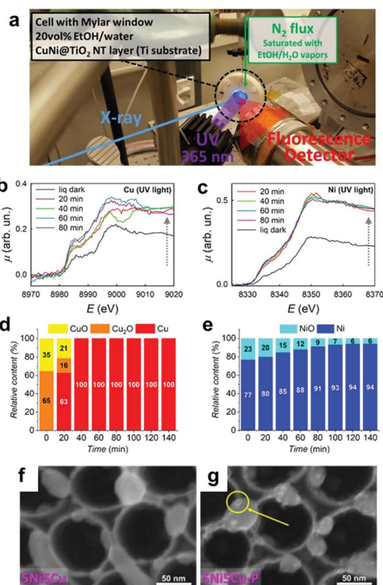
Fig. 13 (a) Operando XAS experimental setup; (b) Cu K-edge and (c) Ni K-edge XAS spectra of 5Ni5Cu–TiO 2 in a water–ethanol under UV irradiation for various exposure times; (d) Cu and (e) Ni phase contents determined by operando XAS for 5Ni5Cu–TiO 2 ; SEM images of 5Ni5Cu–TiO 2 (f) before and (g) after photocatalysis (a yellow circle indicates metallic NPs deposited under the UV irradiation). Adapted with permission from ref. 171; copyright 2020 ACS.
