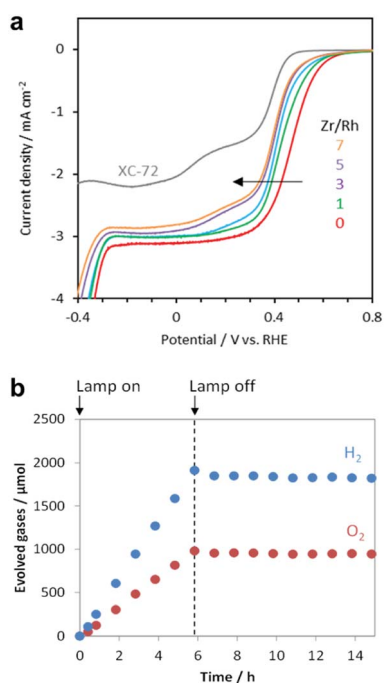
Fig. 12 (a) Current–potential curves of RhZrO x (Zr/Rh: 0–7 w/w)-loaded carbon supports in O 2 -saturated 1 M Na 2 SO 4 (pH 7); (b) gas evolution over time by RhZrO x /SrTiO 3 :Al (Rh = 0.1 wt% and Zr = 0.5 wt% vs. SrTiO 3 : Al) during and after light irradiation (300 W Xe lamp). Adapted with permission from ref. 169; copyright 2020 RSC.
