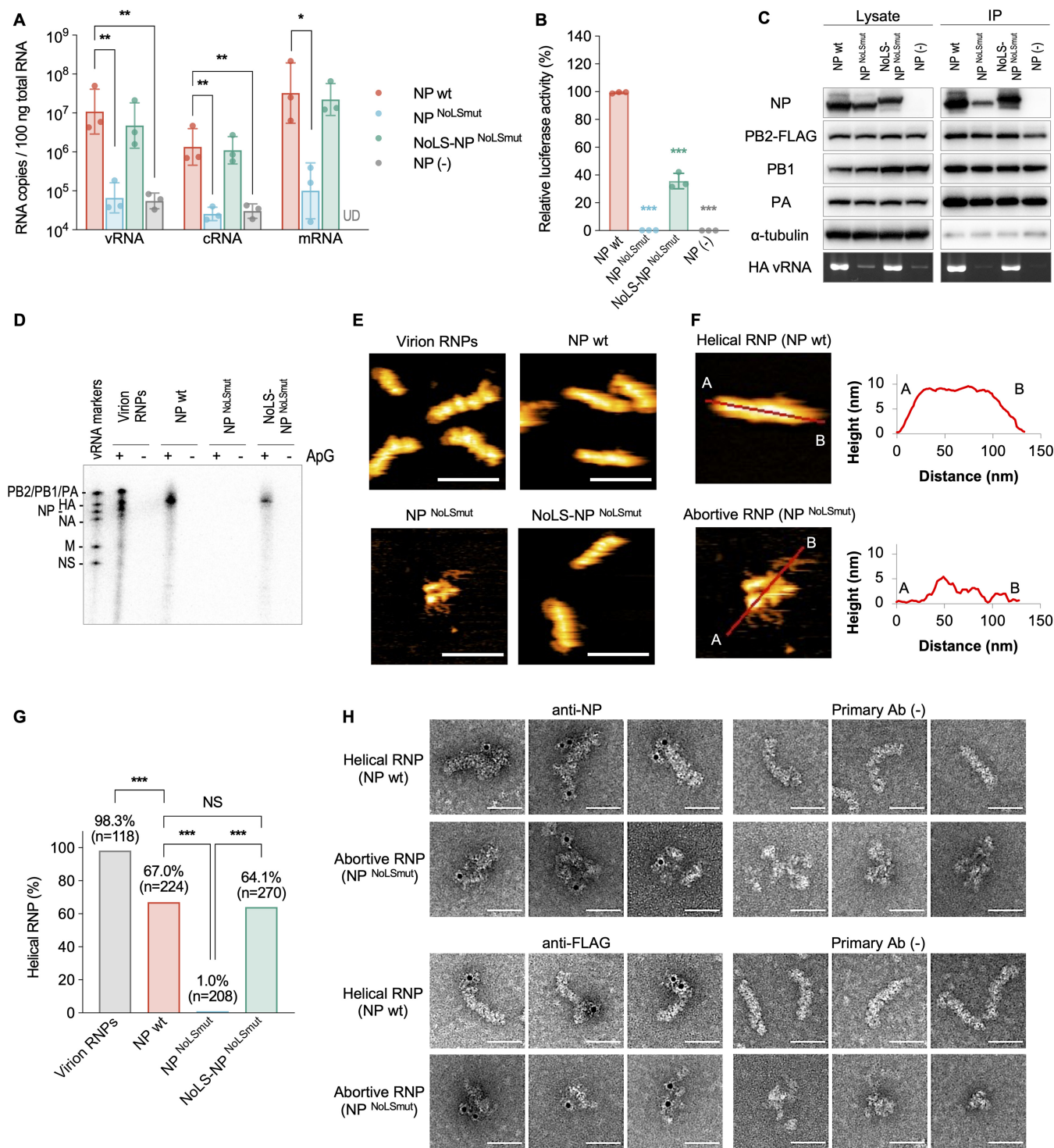
FIG 2 Nucleolar localization of NP is essential for functional and helical RNP formation. (A) Replication and transcription efficiencies of the reconstituted RNPs, measured by strand-specific RT-qPCR. HEK293T cells were transfected with PB2, PB1, PA, and NP proteins and HA vRNA expression plasmids, and total RNA was extracted at 48 h posttransfection (hpt). Their HA vRNA, cRNA, and mRNA copy numbers were compared using a Kruskal-Wallis test with Dunn's test (*, P < 0.05 ; **, P < 0.01 ; UD, undetected). The data are presented as geometric means \pm the standard deviations (SD) of three independent experiments with two RT-qPCR assays. (B) Polymerase activity of the reconstituted RNPs in HEK293 cells, measured by minigenome assay. Relative firefly luciferase activities were compared to that of the RNPs reconstituted with NP wt using one-way ANOVA with Dunnett's test (***, P < 0.001 ). The data are means \pm the SD from three independent experiments with duplicate wells. (C) Reconstruction and immunoprecipitation of RNPs. The RNPs were reconstructed by transient expression of PB2-FLAG, PB1, PA, and NP proteins and HA vRNA in HEK293T cells, followed by immunoprecipitation using anti-FLAG antibody-conjugated agarose beads. The viral proteins and \alpha -tubulin were immunoblotted. The full-length HA vRNA was detected by RT-PCR. Representative images from three independent experiments are shown. (D) In vitro transcription of the reconstructed RNPs. Nascent viral RNA was transcribed in vitro with ApG primer and detected by autoradiography. RNPs derived from virion (virion RNPs) were used as the control. vRNA markers are (Continued on next page)
