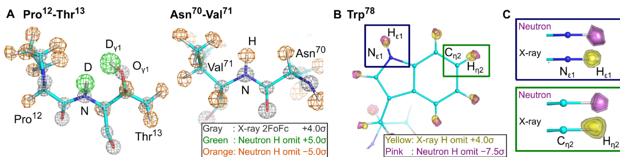
Fig. 1. Electron and nuclear density maps of oxidized HiPIP. (A) Electron and nuclear density maps around the peptide bond between Pro 12 and Thr 13 and between Asn 70 and Val 71 . The 2F_{obs} - F_{calc} electron density map is shown in gray at a contour level of +4\sigma . The F_{obs} - F_{calc} hydrogen omit nuclear density map is shown in green and orange at a contour level of +5\sigma and -5\sigma , respectively. (B) Difference between the center of electron density and nuclear density of the indole ring of Trp 78 . The F_{obs} - F_{calc} hydrogen omit electron density map and F_{obs} - F_{calc} hydrogen omit nuclear density map are shown in yellow ( +4\sigma ) and pink ( -7.5\sigma ), respectively. (C) Close-up view of N_{\epsilon 1}-H_{\epsilon 1} and C_{\eta 2}-H_{\eta 2} of Trp 78 . The F_{obs} - F_{calc} hydrogen omit electron density map and F_{obs} - F_{calc} hydrogen omit nuclear density map are shown in yellow ( +4.5\sigma , +4\sigma , and +3.5\sigma ) and pink ( -8\sigma , -7.5\sigma , and -7\sigma ), respectively.
