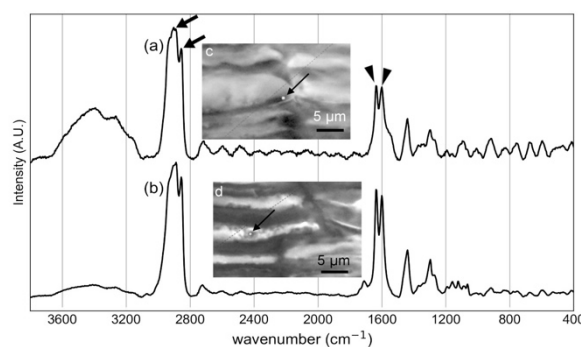
Fig. 7 Raman spectra (a, b) of birch cork acquired from the point indicated by arrows in brightfield micrographs (c, d) of a transverse section. Arrows in (a) indicate CH stretching bands that stem from the suberin aliphatic domain. Arrowheads indicate peaks that stem from the aromatic ring.
