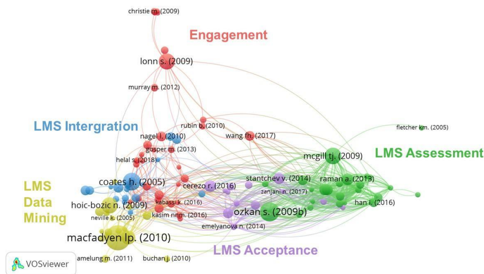
Figure 5: Bibliography coupling map of LMS in HE (20 times, 106 publications)
