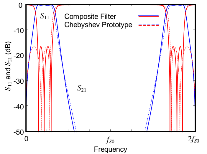
Fig. 5. Frequency response of composite filter after passband match.
