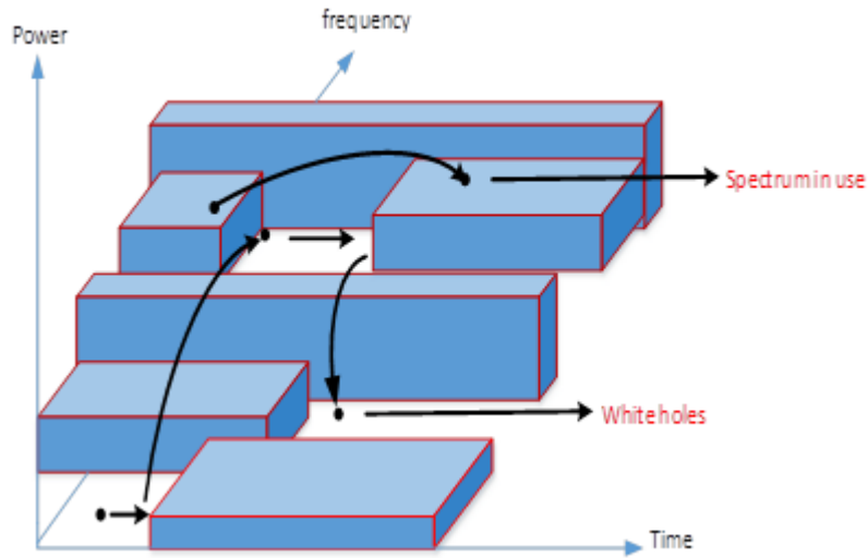
Figure 5: An illustration of DSA (Chiwewe et al., 2015; Yau et al., 2009)
