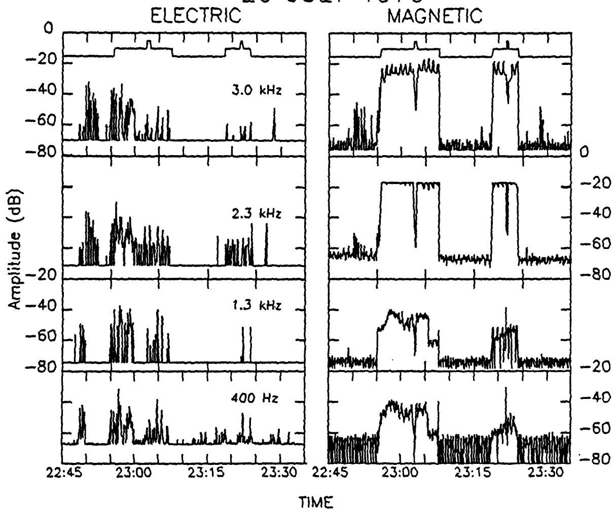
Figure 2. Narrowband Electric and Magnetic Receiver Data for 20 July 1979
