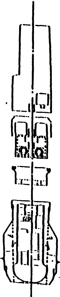
Figure 3. HMS Lancaster profile. Locations 1 and 2 are the metal box and hangar deck roof where measurements were conducted.
