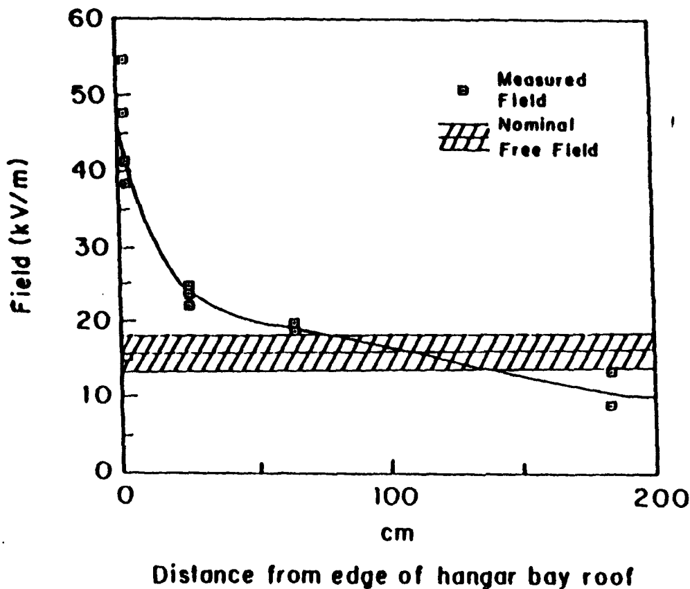
Figure 6. Field measurements on roof of hangar bay along the centerline. The squares are the measured fields and the line is a guide to the eye. The nominal peak free field value indicated by the hatch line was 16.1 \pm 2.3 kV/m.
