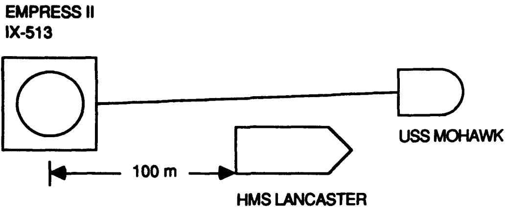
Figure 2B. Test Configuration with HMS LANCASTER between EMPRESS II and USS MOHAWK.
