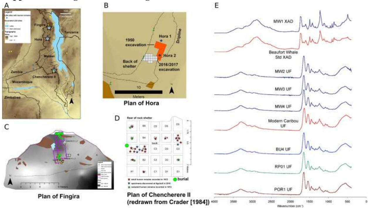
Figure S1. Archaeological context and dating of newly reported human remains from Malawi. Related to Figure 1. A) Locations of the three sites in Malawi. B) Plan of the Hora rock shelter showing locations of the original Hora 1 (male) and Hora 2 (female) burials relative to new excavations from 2016. C) Plan of Fingira Cave showing locations of human remains recovered in 1966 (green dots) and 2016 (green stars). D) Plan of Chencherere II rock shelter redrawn from Crader (1984), showing approximate locations where human remains were recovered in 1972 (red and green stars), and the approximate locations of the remains sampled from Nguludi for this study (blue stars). E) Ultrafiltered collagen FTIR spectra for three individuals from Malawi (MW2 = UCIAMS-186346, MW3 = UCIAMS-18647, MW4 = UCIAMS-186348) compared to well-preserved standards and samples (Modern Caribou, BU4, RP01, POR1). These samples show the typical features for well-preserved collagen. The top of the figure shows the FTIR spectra for a single XAD purified sample (MW1 = PSUAMS-1734) compared against a well-preserved standard (Beaufort Whale). These data, along with the stable isotopes and C:N ratios, indicate that these samples are well-preserved and that the AMS 14 C dates are reliable.
