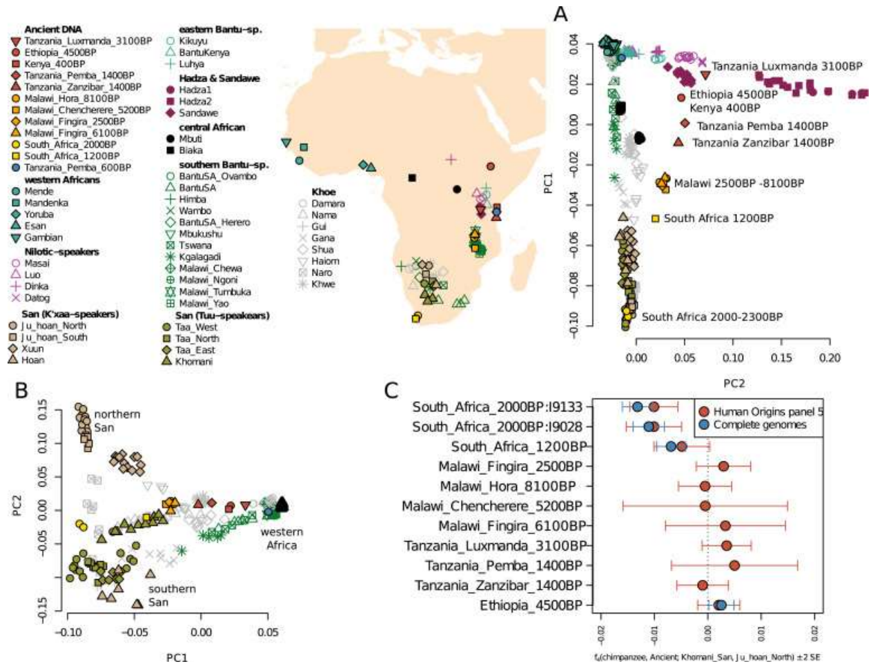
Figure S2. Ancient individuals and African population structure. Related to Figure 1. A) full legend and PC1-PC2 scatter plot (same analysis as Figure 1) with all present-day populations indicated with separate symbols. B) PC1-PC2 computed only with southern African populations (and west African Yoruba). C) Symmetry statistics confirming that ancient individuals from the western Cape region in South Africa are more closely related to southern San such as the Khomani rather than more northern San populations such as the Ju_hoan_North.
