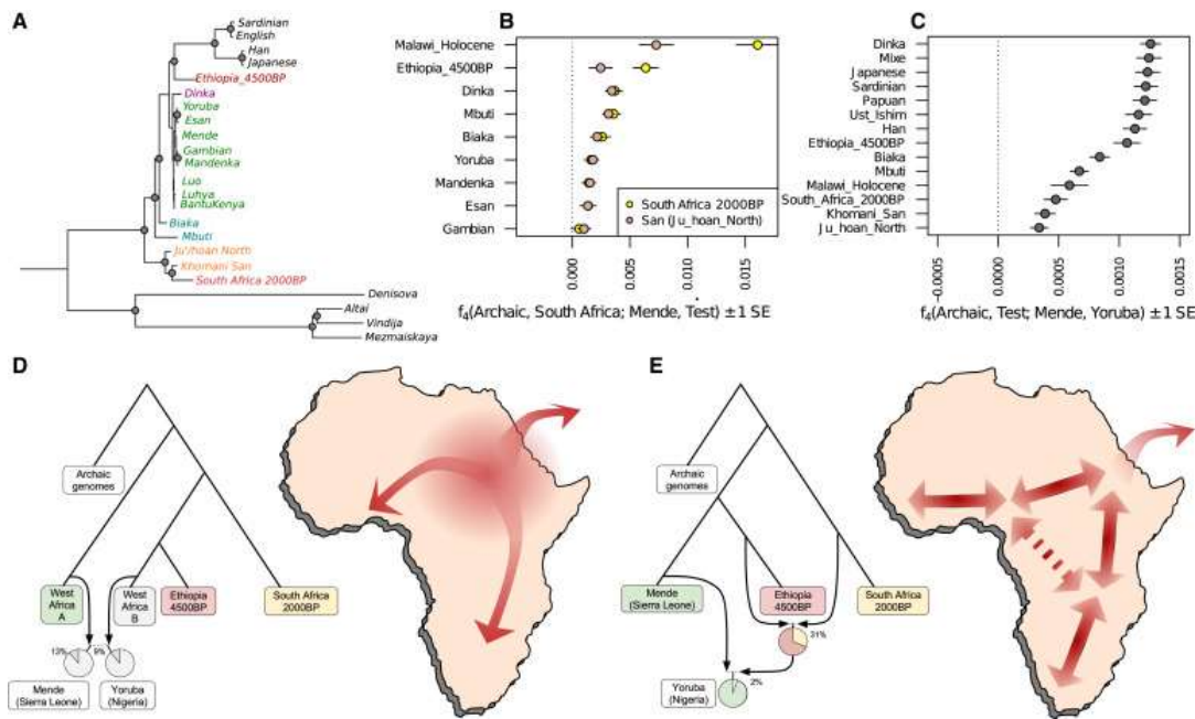
Figure 3. Mixture events in the deeper population history of continental African lineages. A) Maximum likelihood tree of genome sequences from present-day and ancient populations, excluding populations with evidence of asymmetrical allele sharing with non-Africans indicative of recent gene flow ( Table S5 ). Nodes with bootstrap support >95% are indicated with a circle. B) A symmetry test of the hypothesis that ancient southern Africans are an outgroup lineage to other African populations, which can be rejected for most pairs. C) Asymmetry between western African Mende and Yoruba in the 1000 Genomes Project data is maximized in the Yoruba’s excess affinity to eastern Africans and non-Africans, but highly significant also for groups as distant as southern Africans. D) Admixture Graph solution where Mende from Sierra Leone and Yoruba from Nigeria have ancestry from a basal western African lineage. The other source of western African ancestry is most closely related to eastern Africans and non-Africans ( Fig. S5D ), which could be consistent with an expansion from eastern Africa. Note that the exact proportion ‘West Africa A’ ancestry is not well constrained by the model, but the difference between Yoruba and Mende is highly significant (panel C). E) Admixture graph solution where the Yoruba have gene flow from a population related to both southern and eastern Africa, which could be consistent with a more complex pattern of isolation-by-distance in the continent.
