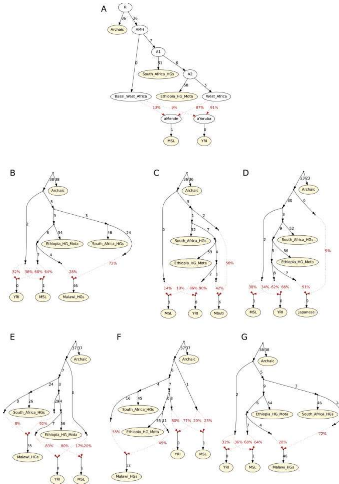
Figure S5. Automatically adding additional populations to a skeleton graph. Related to Figure 3. A) Skeleton graph invoking widespread admixture from a hypothesized ancestral northeast African population. B-D) Best fitting insertion points for Malawi_Hora_8100BP shotgun sequence data (B), Mbuti (C), and Japanese non-Africans (D), in the skeleton graph displayed in (A). For details see Table S6 .
