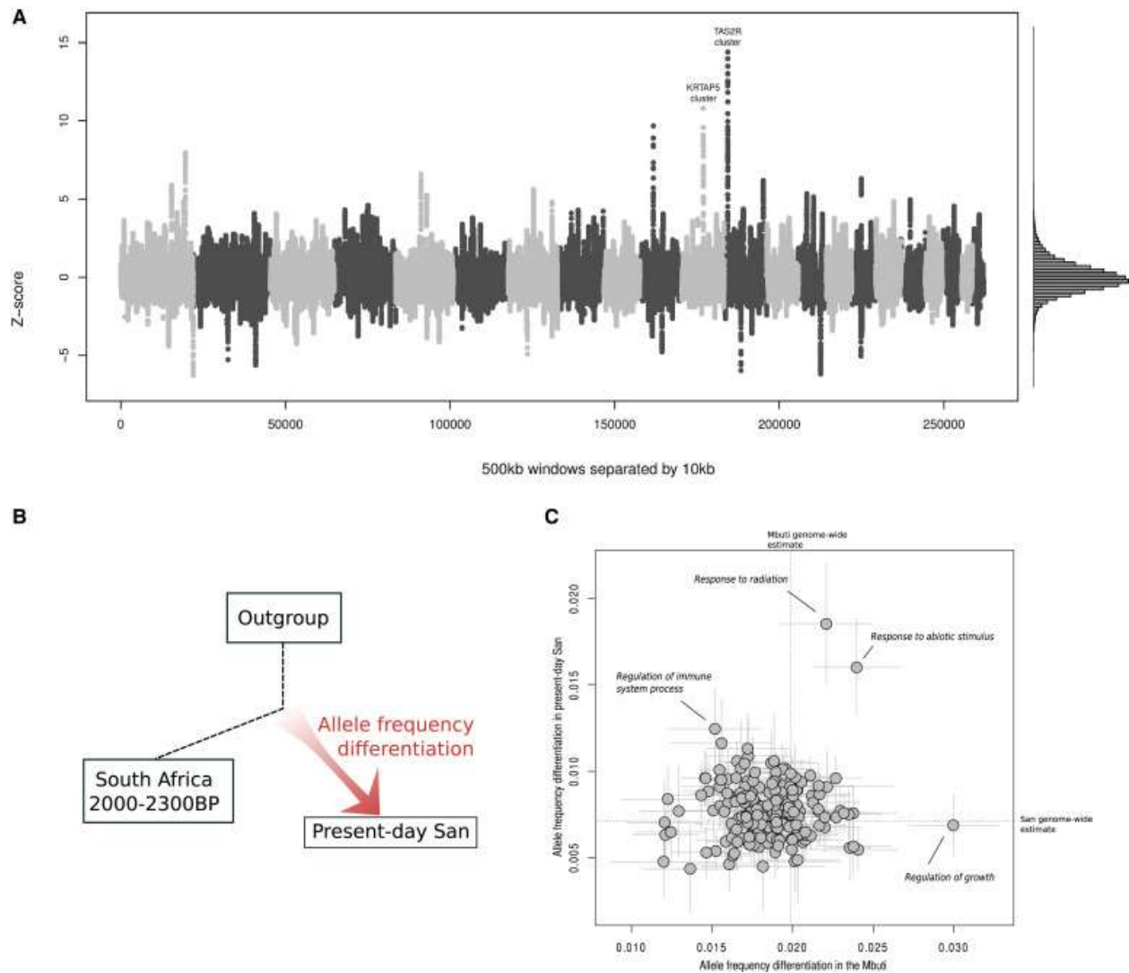
Figure 4. Ancient genomes provide evidence of natural selection in present-day southern African San populations. We computed branch-specific allele frequency differentiation in 6 present-day high-coverage San genomes compared to a pool of two ~2000 BP South African genomes as an outgroup, using two approaches. A) We computed the statistic in windows of 500kb separated by 10kb. We also estimated genome-wide average and standard deviation of the statistic using windows separated by at least 5 Mb, and transformed the genome wide distribution of the sliding windows to be approximately normal (right panel). We observe outliers 15 standard deviations from the mean in a taste receptor gene cluster on chromosome 12, and a secondary peak in the Keratin Associated Protein 4 gene cluster. The outgroup used was 4 Central African Mbuti genomes. See Table 2 for details on all major outlying regions. B) Illustration of the branch-specific allele frequency differentiation approach. C) We computed the statistic and block jackknife standard errors for 208 gene ontology categories with at least 50 genes each (y-axis). The outgroup used was western Africans. As a control to confirm that outlier categories do not show larger magnitudes of allele frequency differentiation across populations, we replaced the present-day San with the central African Mbuti (x-axis).
