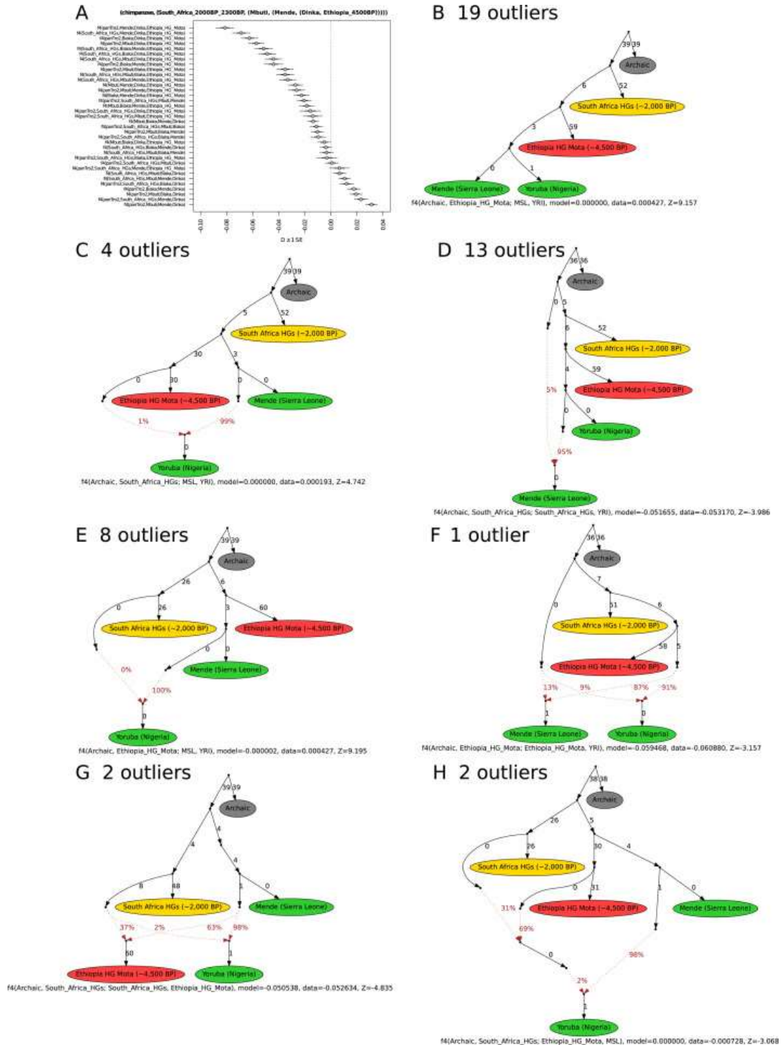
Figure S4. Admixture models of African population history. Related to Figure 3. A) A tree-like model. Tests of all possible triplet topologies predicted to be symmetric by the tree obtained for major African population lineages in the maximum likelihood model in Fig. 3A . B-H) Under each graph we show the outlier f_4 statistic with the greatest Z-score between model and empirical values. When the same group appears twice in an f_4 statistic (e.g. f_4(\text{Archaic, South\_Africa\_HGs; South\_Africa\_HGs, YRI}) ), this corresponds to an f_3 statistic. Graphs F and H are the most parsimonious fits with only two admixture events.
