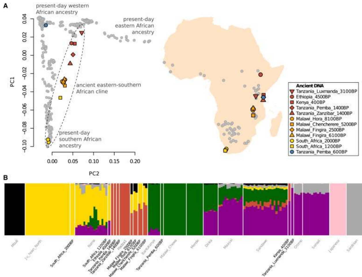
Figure 1. Overview of ancient genomes and African population structure. a) Map of sampling locations in Africa and principal component analysis of all individuals. Present-day individuals are indicated with gray circles. b) Automated clustering of key ancient- and present-day populations (for K=7 cluster components). Present-day populations are labeled in gray.
