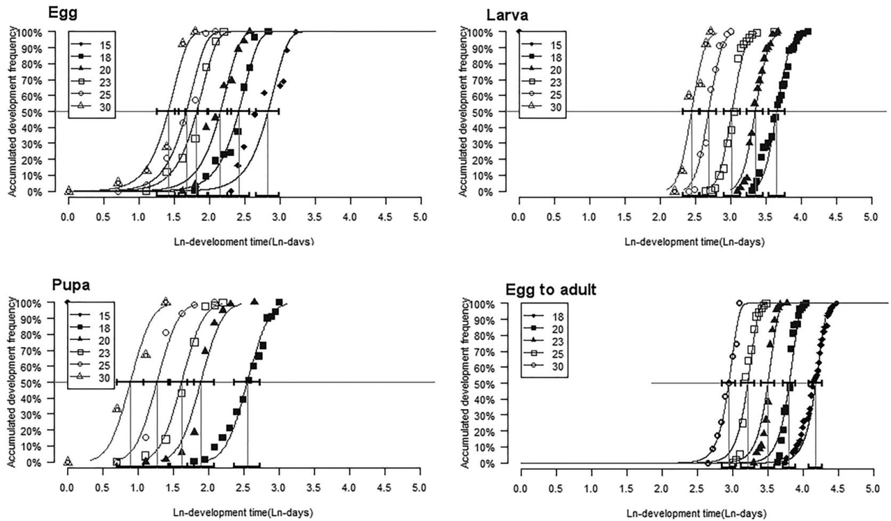
Fig. 1. Cumulative distribution of developmental times of H. hampei egg, larva, pupa and egg to adult. Curves are fitted models: complementary log-log (CLL) model for egg stage and complete development from egg to adult, and probit model for the larva and pupa stages. Bars indicate 95% confidence intervals for median development times estimated from the models.
