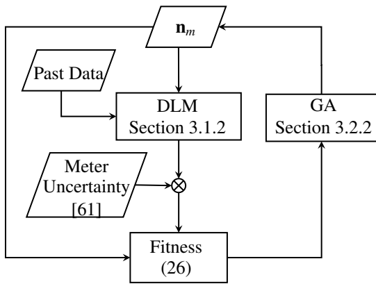
Figure 5: Flow diagram of cross sectional metering sampling designs as in Section 3.2.
