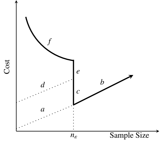
Figure 6: Genetic Algorithm constraint function r(\mathbf{n}) in (27), where n_\varepsilon represents the threshold sample size.
