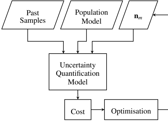
Figure 1: Flow diagram illustrating existing methods [18, 19, 37, 38], where n_m denotes the metering plan.
