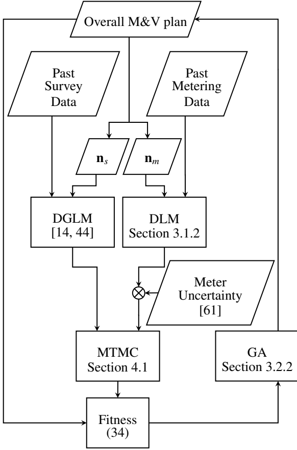
Figure 10: Flow diagram illustrating proposed method for combining metering and surveying data. The metering plan is denoted \mathbf{n}_m , and the sampling plan \mathbf{n}_s .
