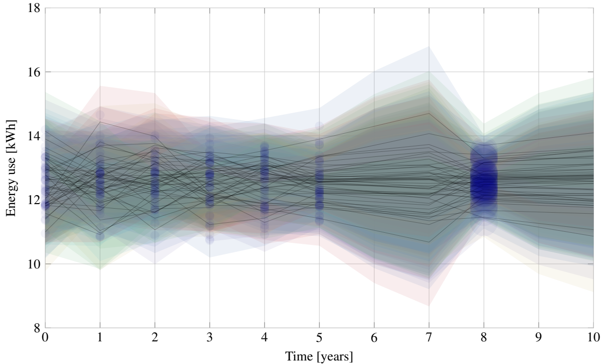
Figure 3: DLM demonstration reflecting true sampling results. Multiple realisations shown.
