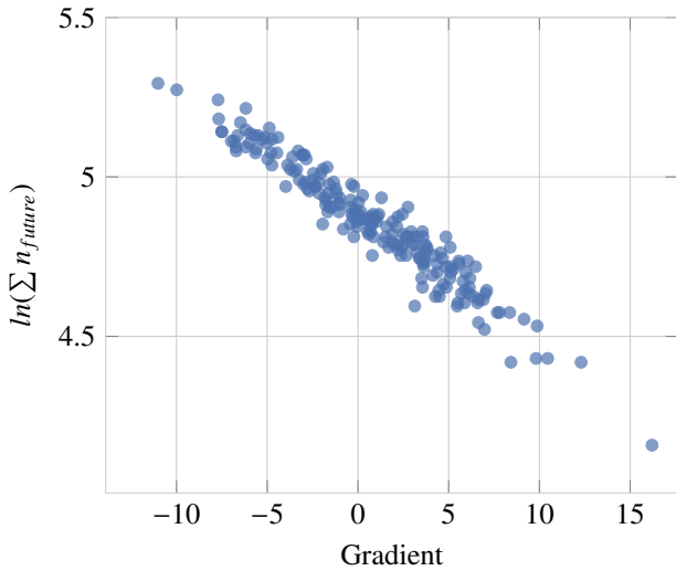
Figure 8: Natural logarithm of the total number of future samples under efficient sampling plans, as a function of the gradients of the regression lines on past samples, e.g. in Figure 7.
