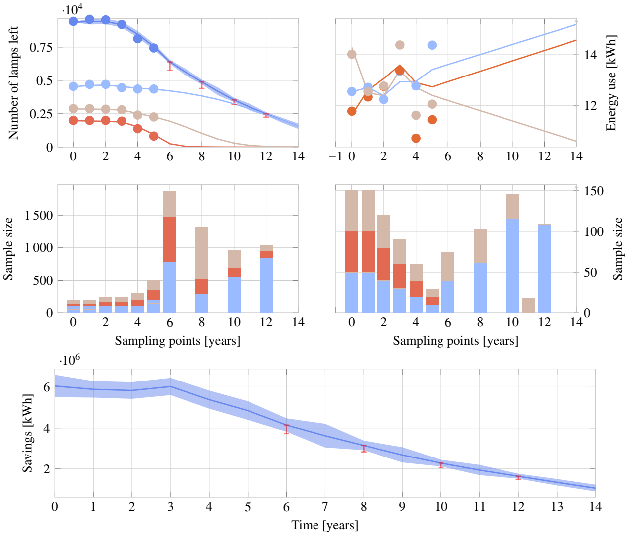
Figure 12: Efficient combined sampling plan using the DLM and DGLM for one random model realisation (Case Study 3). Stratum 1 is in blue, stratum 2 in red, and stratum 3 in brown. Combined values are shown in blue. The 10% error bars are shown in red, and the 90% confidence intervals in light blue.
