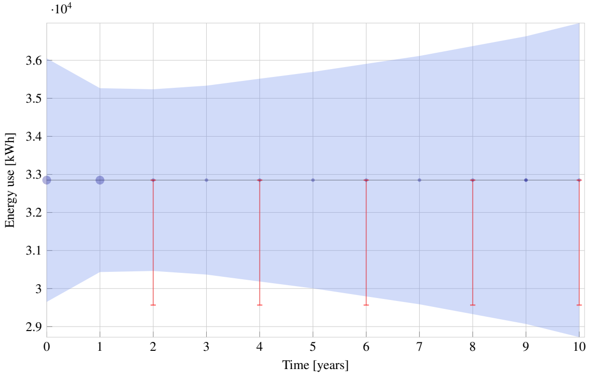
Figure 4: 90% Confidence bounds (shaded) compared to 10% precision limits (red error bars) for previous sampling plan using earlier method [19, 38], analysed by DLM.
