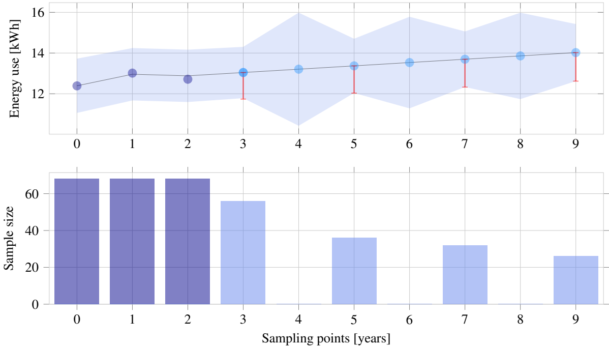
Figure 7: Efficient sampling plan using the DLM for one random model realisation
