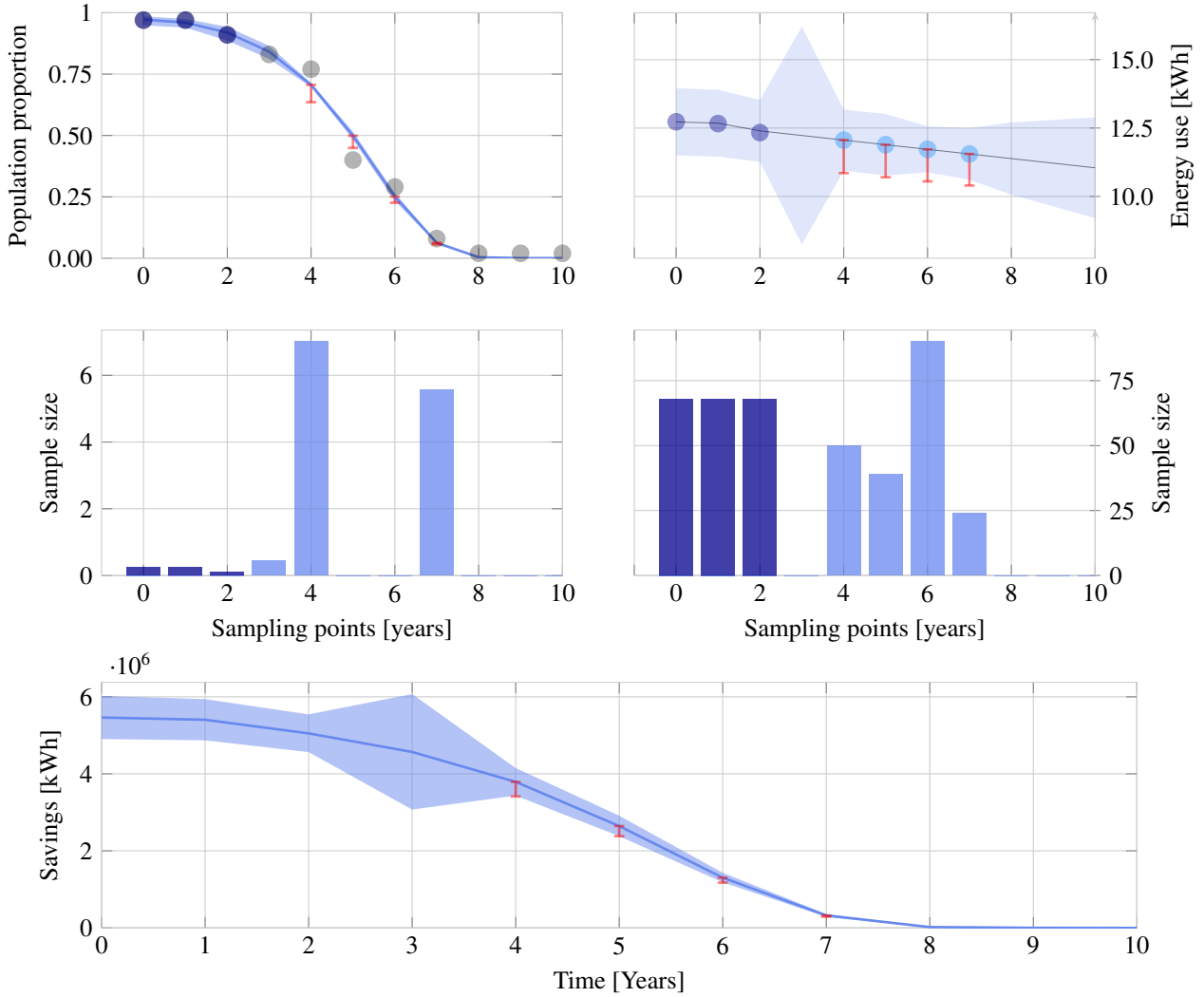
Figure 11: Plot of combined survey sampling (top left) and metering (top right) for a single population (Case Study 2), with the combined savings estimate over time at the bottom. Dark blue indicates past samples, and light blue indicates planned future samples.
