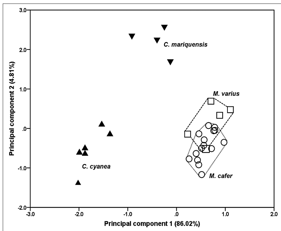
Fig. 5. A biplot derived from principal components analysis of log 10 -transformed craniometric variables, depicting sample variation amongst the 30 shrew individuals along with the first two principal components
