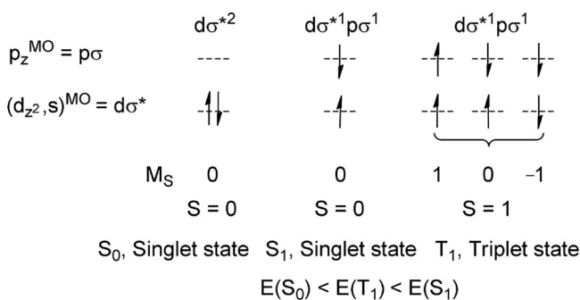
Scheme 7. Microstates and term states for MO configurations dσ* 2 and dσ* 1 pσ 1 in Au 2 (P Λ P) 2 2+ .
