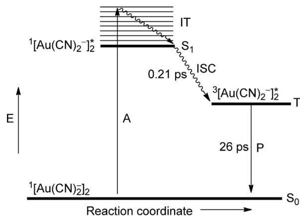
Scheme 9. Simplified Jablonski diagram for the excitation and emission of the dimer [\text{Au}(\text{CN})_2]_2 . A = absorption; IT = internal transition; ISC = intersystem crossing; P = phosphorescence.
