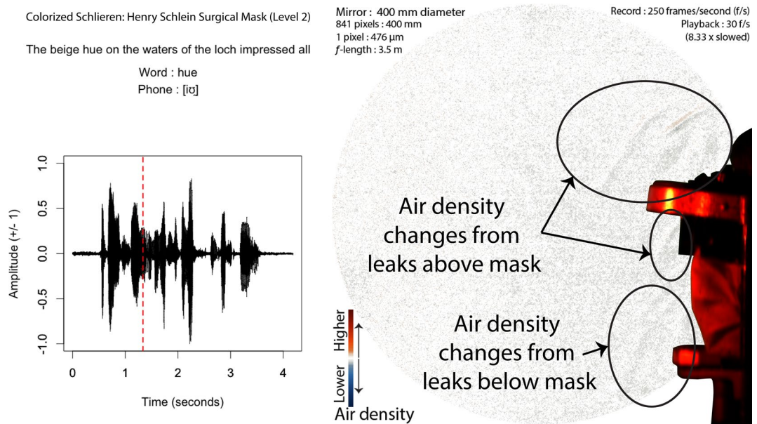
Figure 8. Audio and Schlieren of speech with a tightly fitting surgical mask (Frame 334, 1st block, Henry Schlein surgical mask [level 2]). Air slowly flows out above the eyes, floating out and upward continuously. The red-dashed line in the audio waveform indicates the timing of the schlieren frame.
