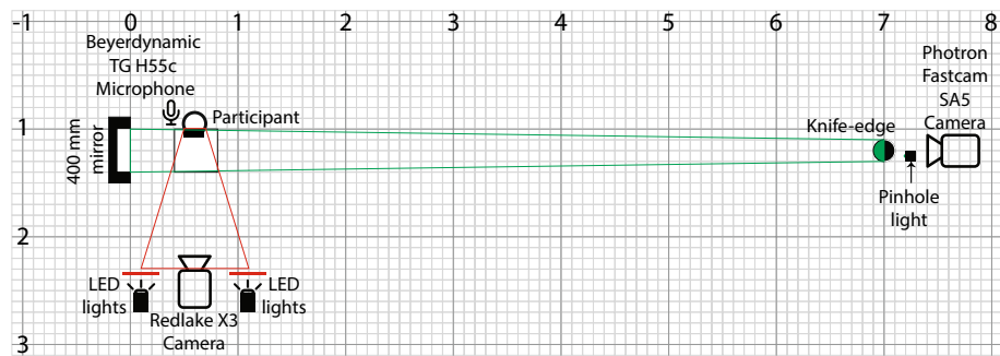
Figure 1. Schematic of schlieren and video setup, to scale in a 0.1 m grid.
