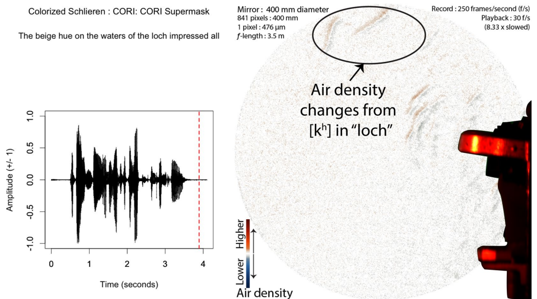
Figure 6. Audio and Schlieren of speech through a porous face mask (Frame 973, 1st block, CORI Supermask). Image from 1,496 ms after the release burst for the [k h ] in "loch". Note that the k's puff has moved slow enough that it floated up to the top of the mirror's span, compared to nearly straight across as in Fig. 4. The red-dashed line in the audio waveform indicates the timing of the schlieren frame.
