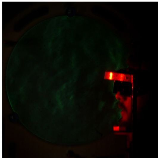
Figure 2. Video frame of Schlieren imaging—frame 2001, no-mask image, first phrase.
