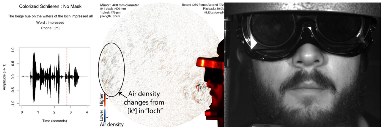
Figure 4. Audio, Schlieren, and Video of speech without a face mask (Frame 691, 1st block, no face mask). Image from 337 ms after the lip opening and release burst for the [k^h] in “loch”. The k 's puff spans the entire length of the mirror, past 35 cm of distance from the lips of the speaker. The red-dashed line in the audio waveform indicates the timing of the video and schlieren frames.
