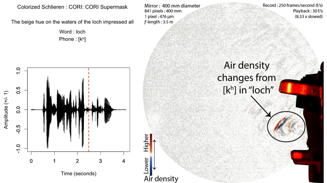
Figure 5. Audio and Schlieren of speech through a porous face mask (Frame 621, 1st block, CORI Supermask). Image from 88 ms after the release burst for the [k h ] in "loch". Note that the k's puff is smoother and less well-defined than the one in Fig. 2, but still has eddies that change air-density across the span of the puff. The red-dashed line in the audio waveform indicates the timing of the schlieren frame.
