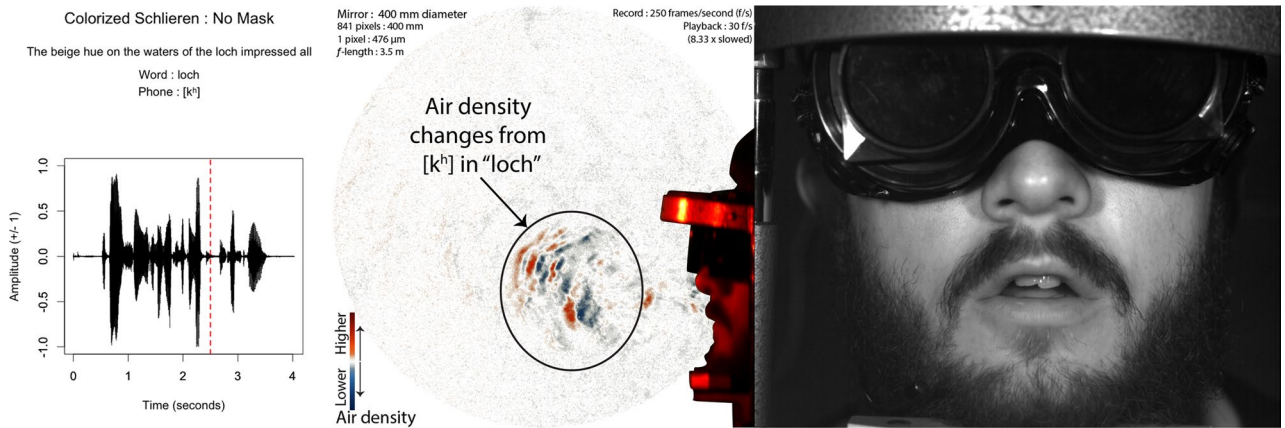
Figure 3. Audio, Schlieren, and Video of speech without a face mask (Frame 625, 1st block, no face mask). Image from 73 milliseconds (ms) after the lip opening and release burst for the [k^h] in “loch”. Note that the k 's puff is strong and well-defined, with eddies that change air-density across the span of the puff. The red-dashed line in the audio waveform indicates the timing of the video and schlieren frames used in this image.
