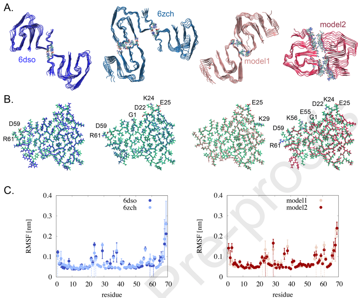
Figure 4. Structure and conformational dynamics from MD simulations. (A) Simulation snapshots of the four fibril structures after 100 ns: 6dso, 6zch, model 1 and model 2. Residues at the protofilament interface are shown in licorice representation. Interfaces involve the following amino acids; 6dso: D59, R61; 6zch: G1, D22, K24, E25; model 1: E25, K29; model 2: G1, D22, K24, E25, E55, K56, D59, R61. (B) Superposition of one central chain of simulated structures after 100 ns and the experimental cryo-EM structure 6dso (shown in green). (C) RMSF averaged over each residue for the experimental cryo-EM structures 6dso and 6zch (left) and the two models with alternative interface (right). Error bars correspond to standard deviations. Dashed vertical lines indicate the residues at the interface.
