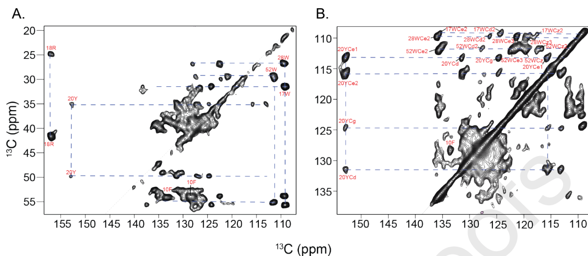
Figure 5. Aromatic region of the 2D ^{13}\text{C},^{13}\text{C} (DARR) correlation spectrum obtained for SAA fibrils. The spectral region containing (A) aliphatic-aromatic and (B) aromatic-aromatic cross-peaks. Distinct resonances for Y20-C \epsilon 1 and C \epsilon 2 chemical shifts suggest that the aromatic ring of Y20 is rigid. At the same time, the aromatic spin systems of W17, W28, and W52 are well resolved, while H36 and H72/H84 cannot be observed.
