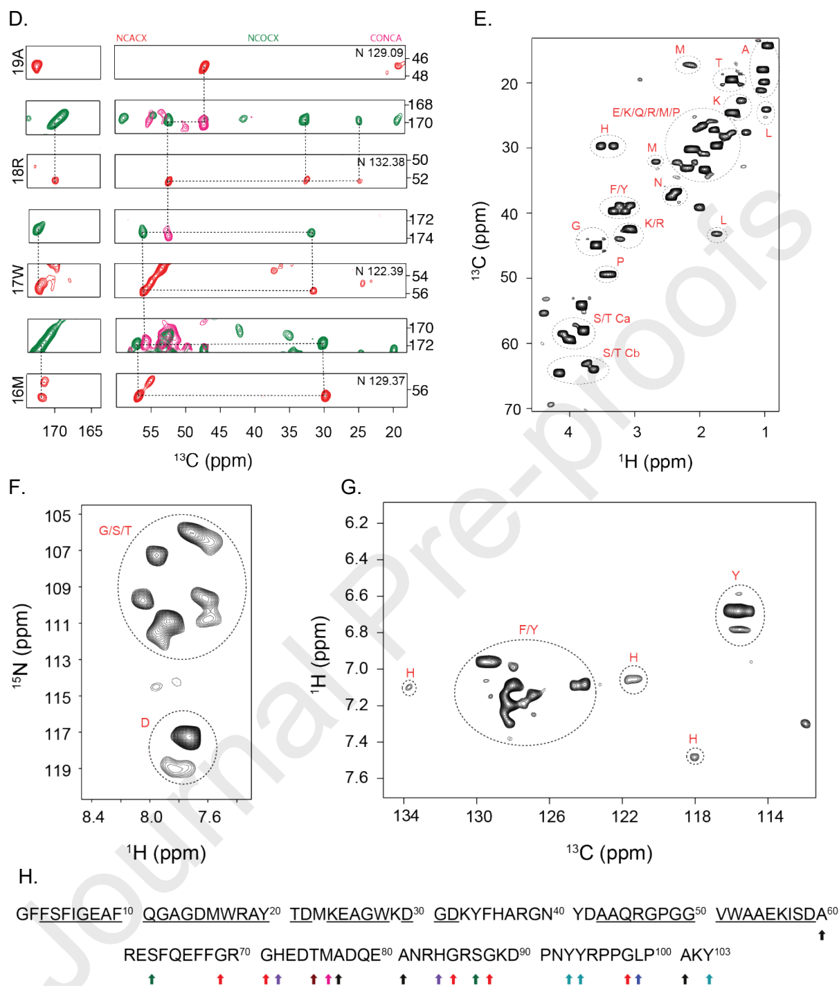
Figure 2. Structural characterization of SAA fibrils using MAS solid-state NMR. (A) 2D - ^{13}\text{C} , ^{13}\text{C} DARR and (B) 2D - ^{15}\text{N} , ^{13}\text{C} correlation spectra of SAA fibrils with assignments. Chemical shifts are deposited in BMRB under the accession code 51285. SC indicates cross peaks originating from side chain resonances. (C) Secondary chemical shifts and \beta -sheet propensity for SAA fibrils obtained from solid-state NMR. (D) 2D strip plots showing sequential connectivities for residues M16-A19 in SAA fibrils from 3D NCACX, NCOCX, and CONCA experiments (represented in red, green and magenta, respectively). (E, F, G) Proton detected ^1\text{H} , ^{13}\text{C} INEPT correlation spectrum, carbon detected ^1\text{H} , ^{13}\text{C} INEPT correlation spectrum, and proton detected ^1\text{H} , ^{15}\text{N} INEPT correlation spectrum, respectively, recorded for a SAA fibril sample in a MAS solid-state NMR rotor. Only dynamic residues are observable in these experiments. Tentative assignments are indicated with dashed circles. Average random coil chemical
