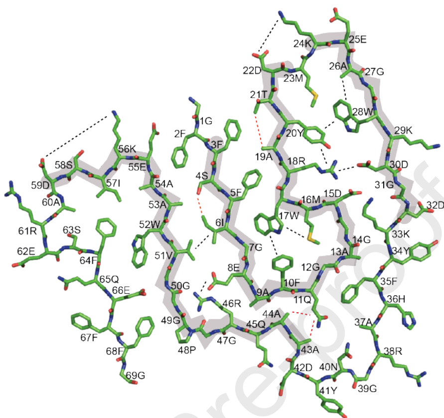
Figure 3. Comparison of the SAA fibril topology from solid-state NMR and cryo-EM. (A) Secondary structure elements of SAA fibrils from solid-state NMR and cryo-EM (Liberta et al., 2019a; Bansal et al., 2021). (B) Long-range distance contacts in SAA fibrils were observed in solid-state NMR experiments. The small panels highlight the cross-peaks involving Y20-W28, I6-V51, F10-W17, and R18-D30, respectively. (C) Cryo-EM ex-vivo fibril structure (PDB ID: 6dso). Residues that could be sequentially assigned by MAS solid-state NMR are highlighted in grey. Long-range distance restraints from NMR experiments are indicated by dashed lines.
