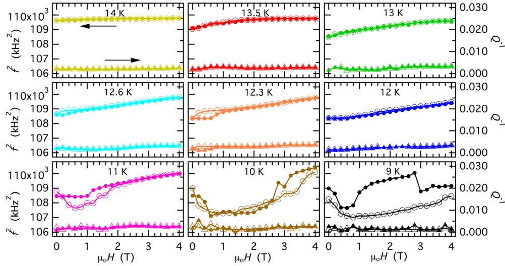
Figure A1. Hysteresis effects and irregular variations at low fields seen in data collected as a function of field ( H/c ) at different temperatures for a resonance which depends predominantly on C_{66} , with frequency in the vicinity of 330 kHz. Filled circles = f^2 with increasing field, open circles = f^2 with subsequent decreasing field, filled triangles = Q^{-1} with increasing field, open triangles = Q^{-1} with decreasing field.
