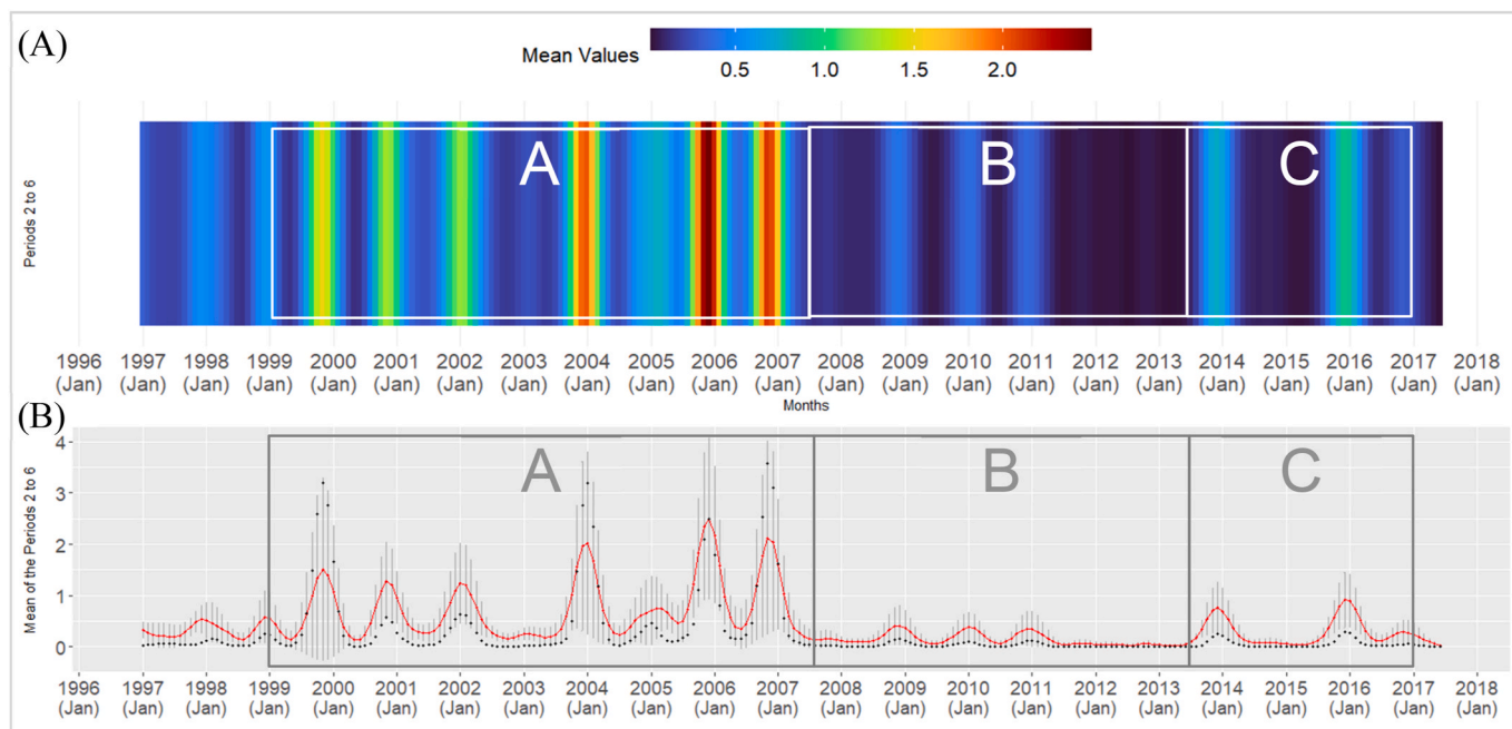
Fig. 9. (A) Calculated mean values of the wavelet analysis (Fig. 8) for the periods two to six. (B) red line presents the mean values of the wavelet analysis (Fig. 8) for the periods between two to six; grey bars represent the standard deviation based on the mean values; black dots show the variation. (For interpretation of the references to colour in this figure legend, the reader is referred to the Web version of this article.)
