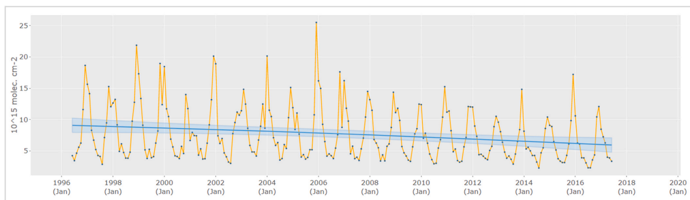
Fig. 6. Time series of the tropospheric \text{NO}_2 monthly mean column values from 1996 to 2017 based on GOME, SICAMCHY, GOME-2A and GOME-2B observations for the area of northern Italy (Latitudes: 44^\circ – 46^\circ , Longitudes: 7^\circ – 14^\circ ). The blue curve represents a cubic spline fit indicating a long-term trend (see text for detail). (For interpretation of the references to colour in this figure legend, the reader is referred to the Web version of this article.)
