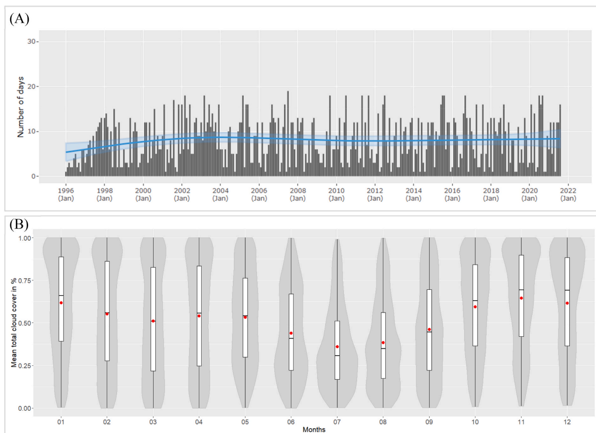
Fig. 1. (A) Available number of days with a total cloud cover of less than 20% for the period 1996–2021 for northern Italy; Blue line represents a cubic spline, (B) Violin plot with included boxplot; Data shows the ERA5 daily total cloud cover for the period from 1996 to 2021 for northern Italy; Red dots represent the mean value and the horizontal lines emphasizes the median (Hersbach et al., 2018). (For interpretation of the references to colour in this figure legend, the reader is referred to the Web version of this article.)
