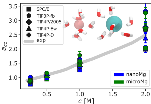
Figure 5. Optimization of ion–ion interactions. Activity derivative a cc as a function of the MgCl 2 salt concentration with the optimized scaling factors for microMg and nanoMg of the various water models (SPC/E, 46 TIP3P-fb, 47 TIP4P/2005, 48 TIP4P-Ew, 49 and TIP4P-D 50 ) (Table 1) and from experiments. 88 The inset shows a representative snapshot of Mg 2+ in interaction with Cl - , including their first hydration shell. This snapshot was taken using microMg (SPC/E) and Cl - parameters from Smith–Dang. 54
