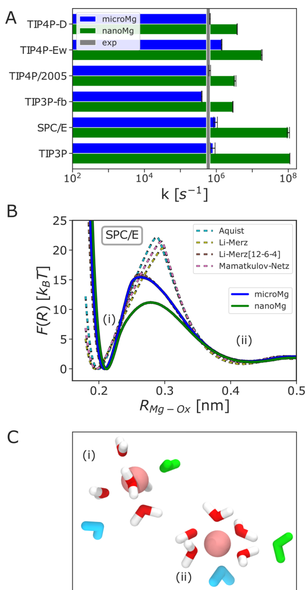
Figure 4. Water exchange in the first hydration shell of Mg 2+ . (A) Kinetic rate coefficients k (eq S3) of microMg (blue) and nanoMg (green) of different water models (SPC/E, 46 TIP3P-fb, 47 TIP4P/2005, 48 TIP4P-Ew, 49 and TIP4P-D 50 ) and for TIP3P from the literature. 26 The gray vertical line indicates the experimental values 73,74 (Table 4). (B) One-dimensional free energy profiles as a function of the distance between Mg 2+ and the leaving water molecule R Mg-Ox for different force fields in combination with SPC/E water. (C) The snapshots show representative conformations in the two stable states: (i) Before exchange: Leaving water (shown in green) is part of the first and entering water (shown in blue) is part of the second hydration shell. (ii) After exchange: Leaving water is in the second hydration shell and the entering water molecule filled the void in the first hydration shell. The snapshots were taken using microMg (SPC/E).
