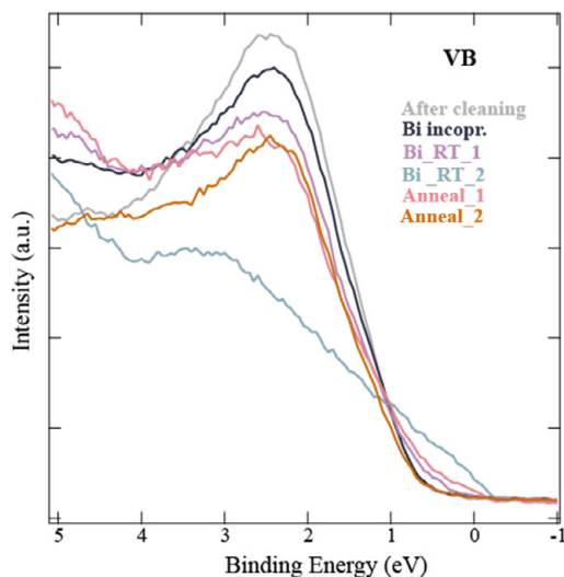
Figure 5.10 Valence band region in XPS spectrum on GaAs(111)B surface upon different Bi deposition and surface treatments. Figure adapted from the supplementary information of Paper II.
