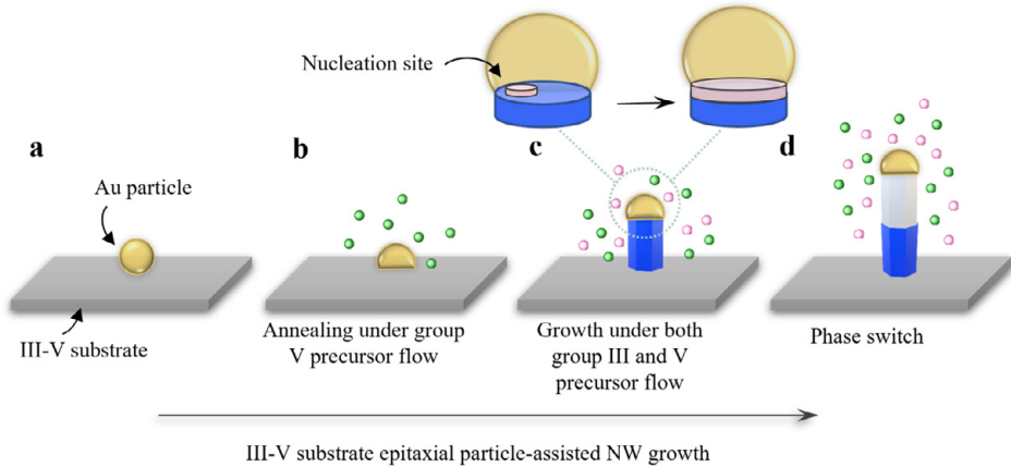
Figure 2.3 The diagram shows the process of nanowire growth with Au particle assisted MOVPE method. a) Au seed is deposited on the substrate; b) Temperature is increased and the group V precursor is flowing in the reactor. c) Introduction of group III and V precursors and growth of the NW. d) NW phase transition by changing the growth parameters.
