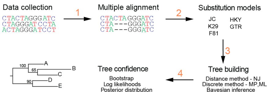
Figure 15. The general phylogenetic inference process.
