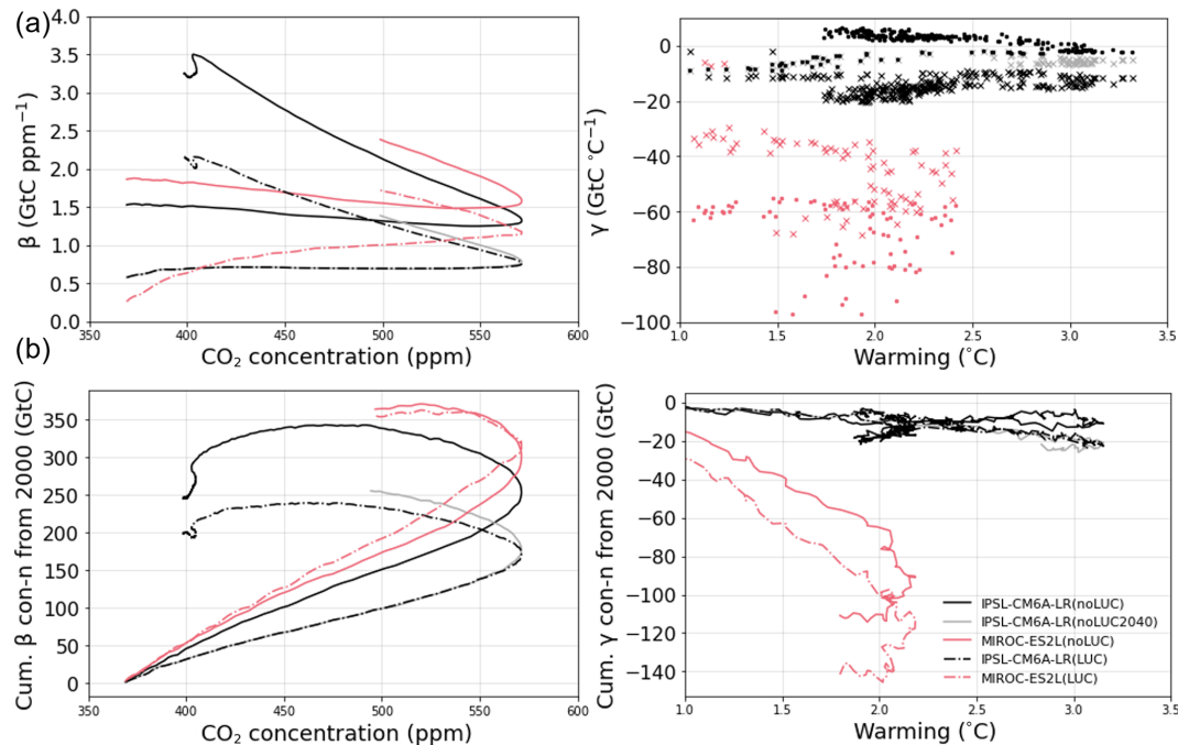
Figure 6. The variation of (a) global \beta_{\text{land}} ( \text{GtC ppm}^{-1} ) and \gamma_{\text{land}} ( \text{GtC } ^\circ\text{C}^{-1} ), and (b) cumulative over 2000–2300 (for IPSL-CM6A-LR) and over 2000–2100 (for MIROC-ES2L) \beta - and \gamma -driven land carbon uptakes with and without LUC. The changes in LUC are given as 9-year moving averages; negative value corresponds to a land sink.
