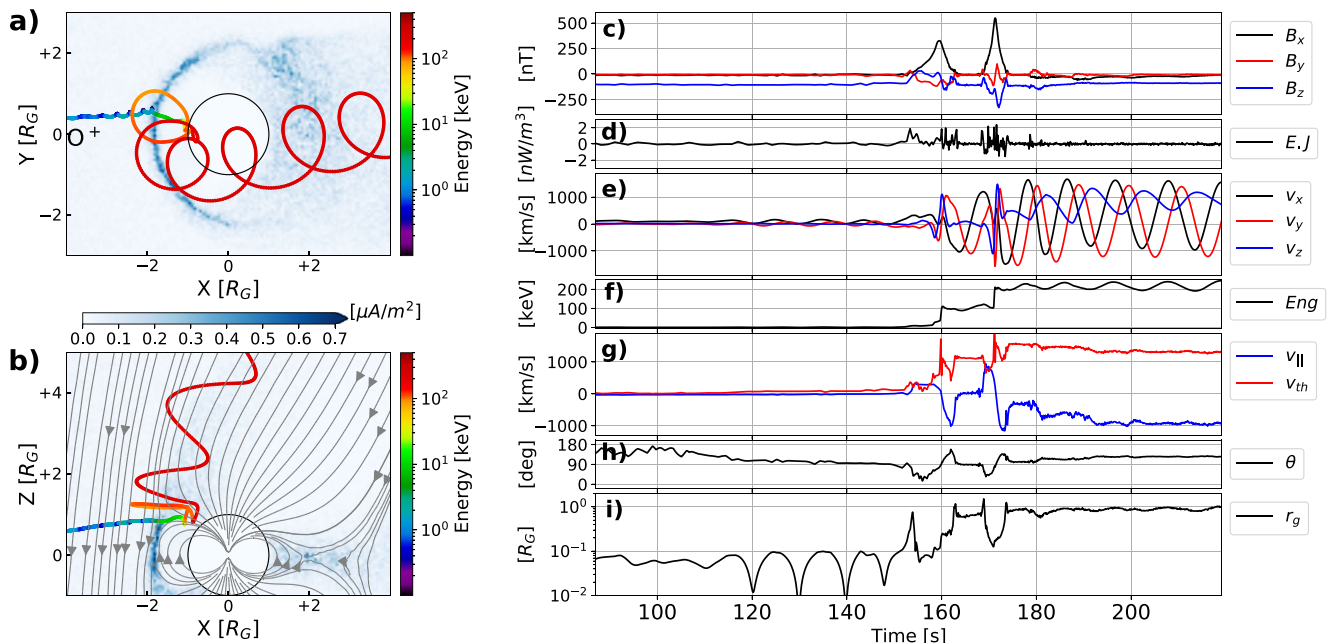
Figure 12. An example of an O^+ ion trajectory that interacts with Ganymede's magnetopause and gains an energy over two orders of magnitude from its initial energy. The figure format is the same as that shown in Figure 10.
