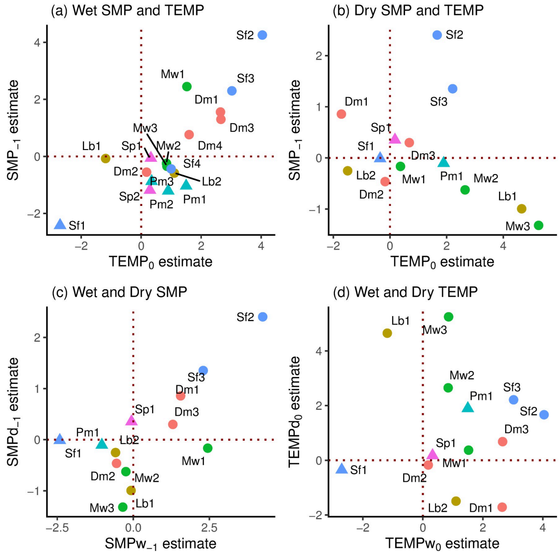
Fig 7. Standardized SMP_{-1} versus TEMP_0 coefficients in relation to one another. Shown are (a) wet [w] and (b) dry [d] periods for the 18 respective 13 trees analyzed for their gthi time-series, and their corresponding dry- and wet-period (c) SMP_{-1} and (d) TEMP_0 values. Symbols as in Fig 6.
