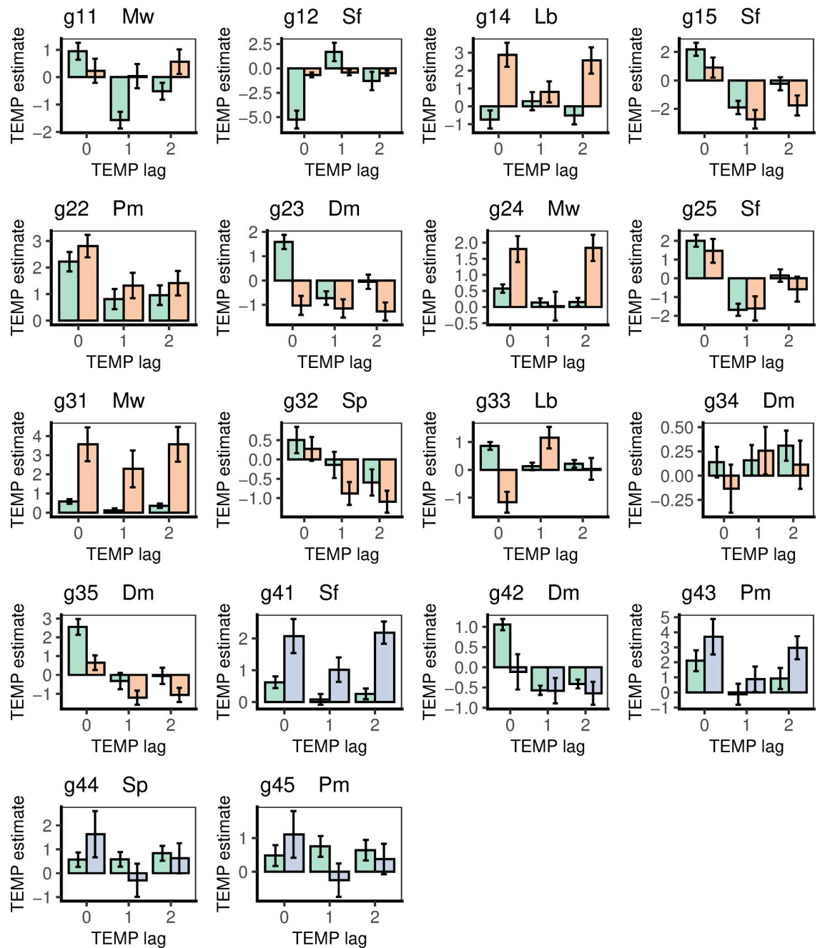
Fig 5. Mean ± SE coefficients (slopes) of gthi regressed on logger temperature (TEMP). TEMP was lagged at 0-, 1- and 2-days, in the wet (green bars) and dry (orange bars) periods, for the 18 trees taken for the time-series analyses. There were no dry-period time-series estimates for station 4, but these are predicted here (blue bars) from the species' relationships to maximal diurnal girth change. Bands are listed in Table 4 with individual tree codes.
