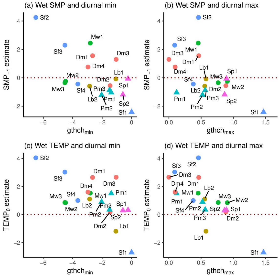
Fig 9. Standardized SMP_{-1} and TEMP_0 coefficients in the wet period in relation to diurnal girth change ( gthch ). In (a, c) the minima, and in (b, d) the maxima, of gthch are used ( n = 18 ). Symbols as in Fig 6.
