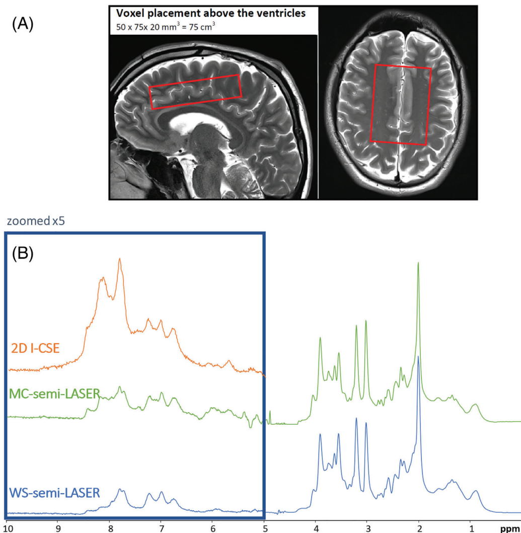
FIGURE 1 Illustration of VOI placement and spectral quality for a representative subject. A) The 75 cm 3 VOI placed centrally above the lateral ventricles with 5 mm spacing. B) Full spectra (downfield and upfield parts) for the semi-LASER-based techniques and the downfield part for frequency-selective 2D I-CSE documenting the overall spectral quality for all three techniques. When comparing noise levels, the differences in total number of scans and differences in different water-scaling have to be kept in mind (number of acquisitions and total scan times: 640, 768, 1280 and 32, 32, 55 min for 2D I-CSE, MC-semi-LASER, and WS-semi-LASER, respectively). I-CSE and MC-semi-LASER scaled with the water signal from MC-semi-LASER, WS-semi-LASER scaled by a reference signal recorded with the same sequence, but without VAPOR. Identical length of the acquired FID, no apodization, downfield part scaled by a factor of 5 compared to the upfield spectra)
