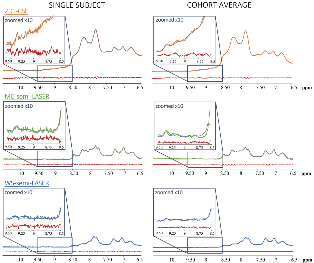
FIGURE 4 Illustration of the last step in model fitting for all three techniques where the parameters are optimized for the downfield part of the spectra only. Experimental (orange, green, and blue) and fitted (gray) spectra are overlaid, while residues (difference between experimental and fitted spectra in red) are plotted with an offset for clarity. Vertical scaling between methods as in Figure 2
