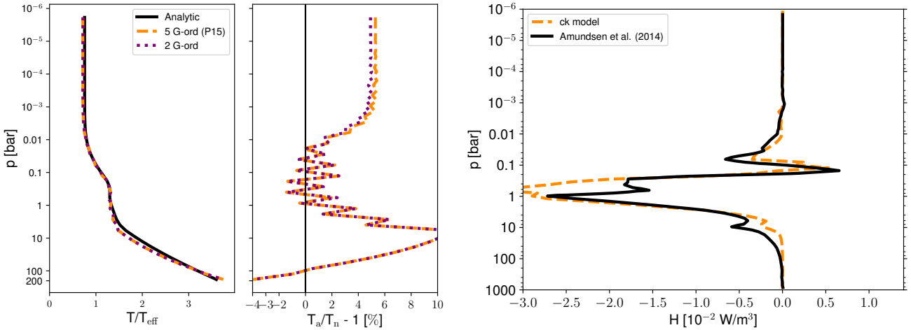
Figure A2. Validation of the semi-grey and corr-k RT set-up. Left: The analytical T-p ( T_a - T_{\text{irr}} = 1288 K, T_{\text{int}} = 500 K, \mu_{\star} = 1/\sqrt{3} ), following the analytical profile of Parmentier et al. (2015) and the equivalent numerical set-up. Right: The correlated-k model instantaneous heating rates, following the Test 2 T-p profile in Amundsen et al. (2014) with the scheme used in the GCM.
