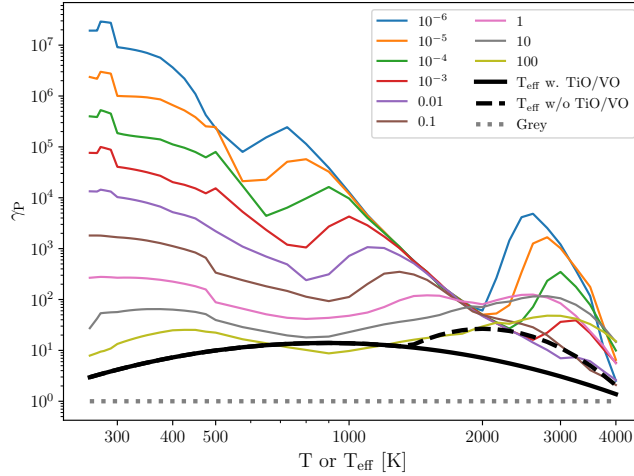
Figure 9. \gamma_P = \kappa_P/\kappa_R calculated from the solar metallicity Freedman et al. (2014) tables. Coloured lines denote the gas pressure in bar. The black lines show the Parmentier et al. (2015) expression as a function of T_{\text{eff}} (solid: with TiO/VO, dashed: w/o TiO/VO). The dotted grey line shows the grey region where \kappa_P = \kappa_R .
