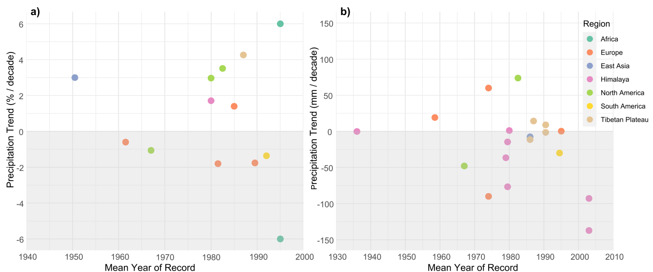
Figure 5. (a) Relative, and (b) absolute changes in mountain precipitation (in situ station studies from SROCC) plotted against the mean year of the respective record. The respective scales are not strictly comparable in terms of vertical stretching as the conversion from absolute to relative change (and vice versa) is dependent upon mean annual precipitation, which varies from place to place.
