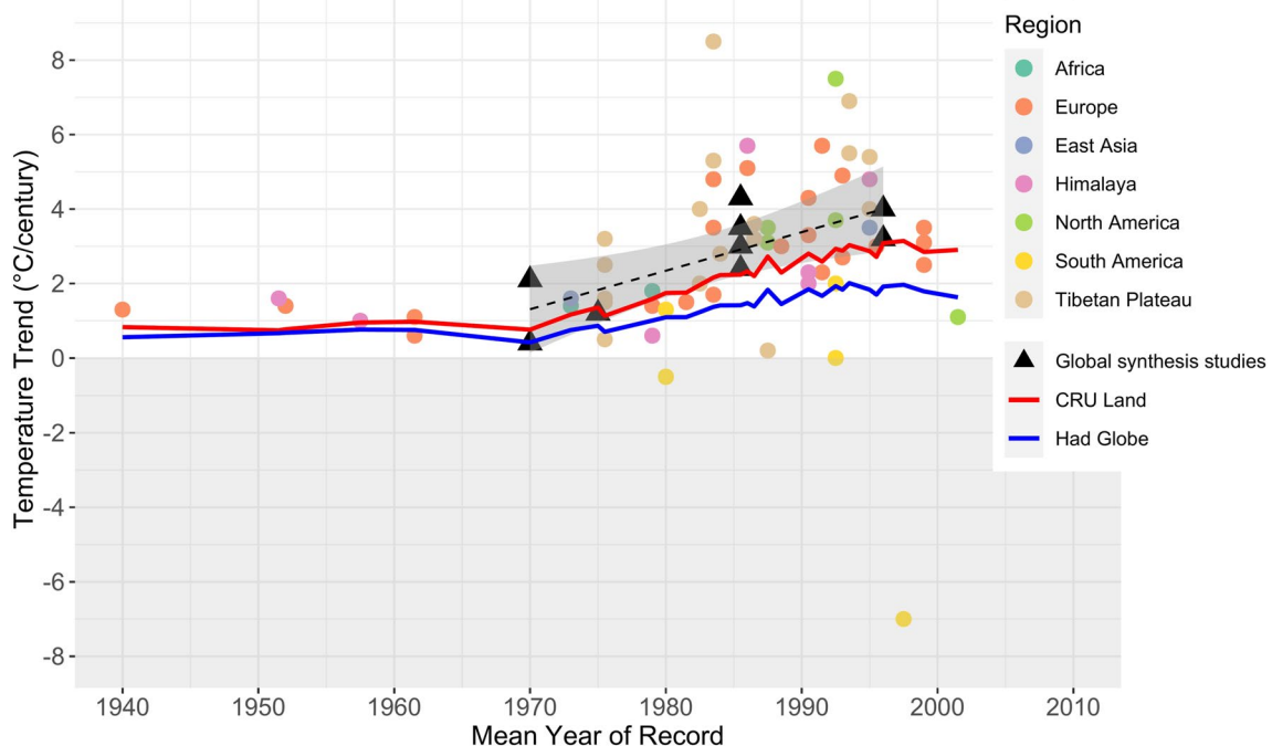
Figure 2. Mean warming rate versus observational record mid-point from all individual studies. Symbol colors indicate the region. Trends from the five global mountain syntheses (>500 stations) are represented by black triangles ( n = 9 ), and the global syntheses best-fit line by the dotted line (linear regression: r^2 = 0.70 , p < 0.01 ). The HadCRUT4 (global land and sea combined) and CRUTEM4 (land surface only) trends for the same period as the mountain studies (variable in length) are represented by the two solid lines. The length of the running mean is indicative of the average length of record upon which the trends in the individual regions are based.
