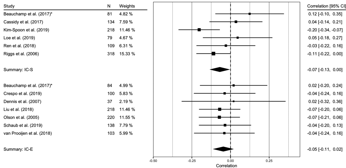
FIGURE 3 Forest plot of moderator analysis for internalizing behavior problems using the a priori defined “Strength/Endurance” (IC-S/IC-E) IC categorization as a subgroup variable. Note. Studies from which multiple effect sizes were used are marked with an asterisk (*)
