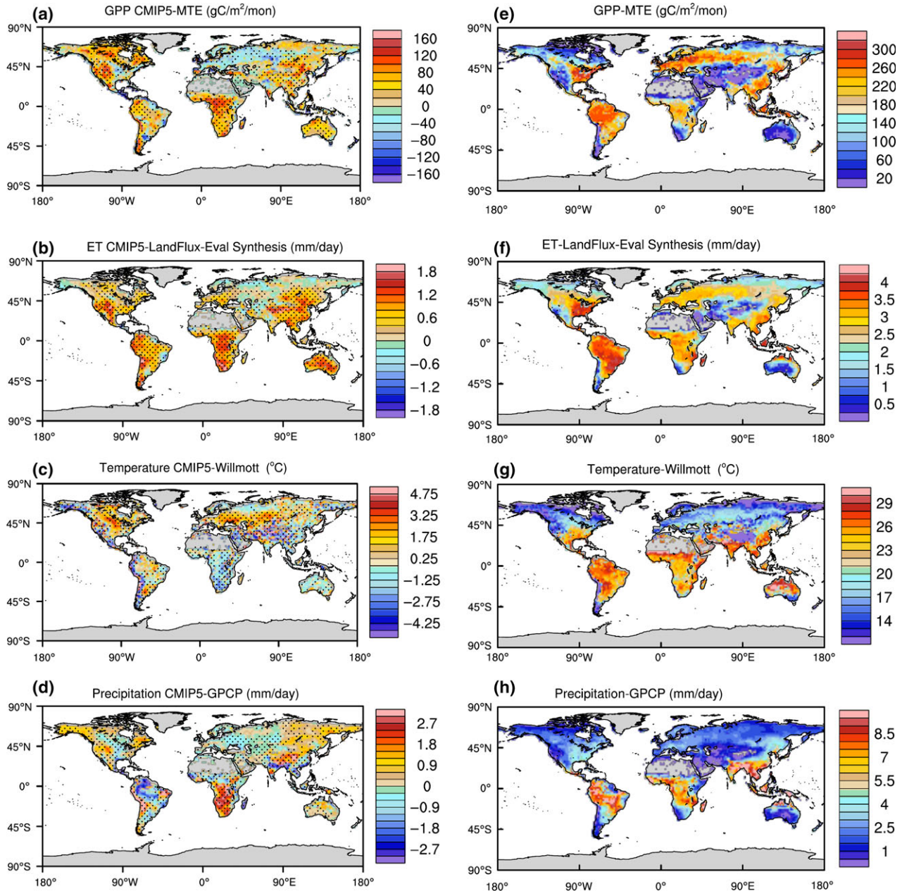
Fig. 2 Mean bias between (a) CMIP5 (multimodel mean) and MTE upscaled GPP ( \text{gC m}^{-2} \text{ month}^{-1} ), (b) CMIP5 (multimodel mean) and LandFlux-Eval ET ( \text{mm day}^{-1} ), (c) CMIP5 (multimodel mean) and University of Delaware temperature ( ^{\circ}\text{C} ) and (d) CMIP5 (multimodel mean) and GPCP precipitation ( \text{mm day}^{-1} ). Stippling is applied over regions where at least 66% of the models (i.e., 13 of 19) agree on the sign of the difference (1989–2005). The spatial distribution of GPP, ET, temperature and precipitation based on reference products is also shown (e–h). Results are shown only for the most productive month.
