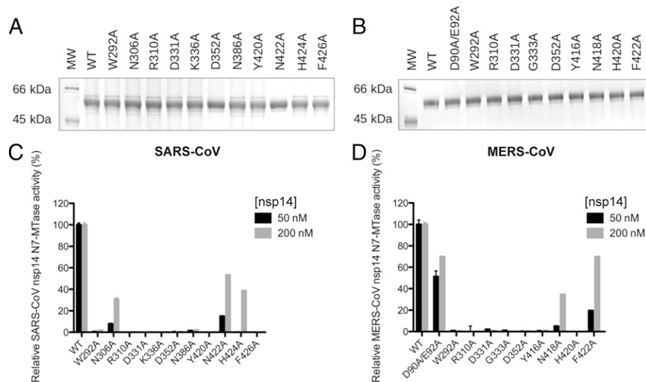
Fig. 3. Expression and in vitro N7-MTase activity of SARS-CoV and MERS-CoV nsp14 mutants. Recombinant SARS-CoV (A) and MERS-CoV (B) wild-type (WT) and mutant nsp14 proteins were expressed in E. coli and purified. Proteins were loaded (2 and 1 \mu g for SARS-CoV and MERS-CoV, respectively) and analyzed using 10% SDS–polyacrylamide electrophoresis gels stained with Coomassie blue. The in vitro N7-MTase activity of SARS-CoV (C) and MERS-CoV (D) nsp14 mutants was determined using an assay with a GpppACCCC synthetic RNA substrate and radiolabeled SAM as methyl donor. Nsp14 concentrations of 50 and 200 nM were used, as indicated. N7-MTase activities were compared to those of the respective wild-type nsp14 controls. For MERS-CoV, ExoN knockout mutant D90A/E92A was included as a control. MW, molecular weight marker.
