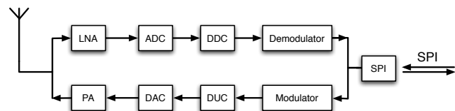
Fig. 3: LoRa Concentrator
