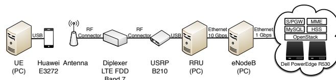
Fig. 11: LTE Setup
