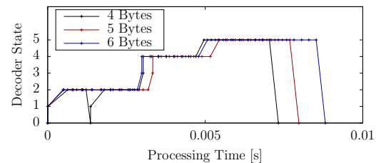
Fig. 12: LoRa Decoder Signal Processing Time
