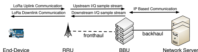
Fig. 7: Cloudified LoRa Network [38]
