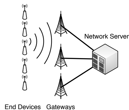
Fig. 1: LoRaWAN Architecture
