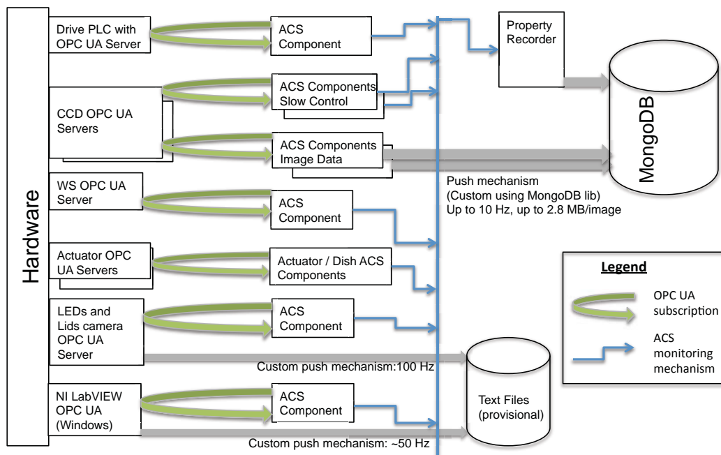
Figure 2. The MST prototype data flow, dominated by the CCD data. The standard OPC UA subscription is used to synchronize the slow control data in the ACS components. The ACS monitoring mechanism consists of both a time-triggered and value change-triggered polling.
