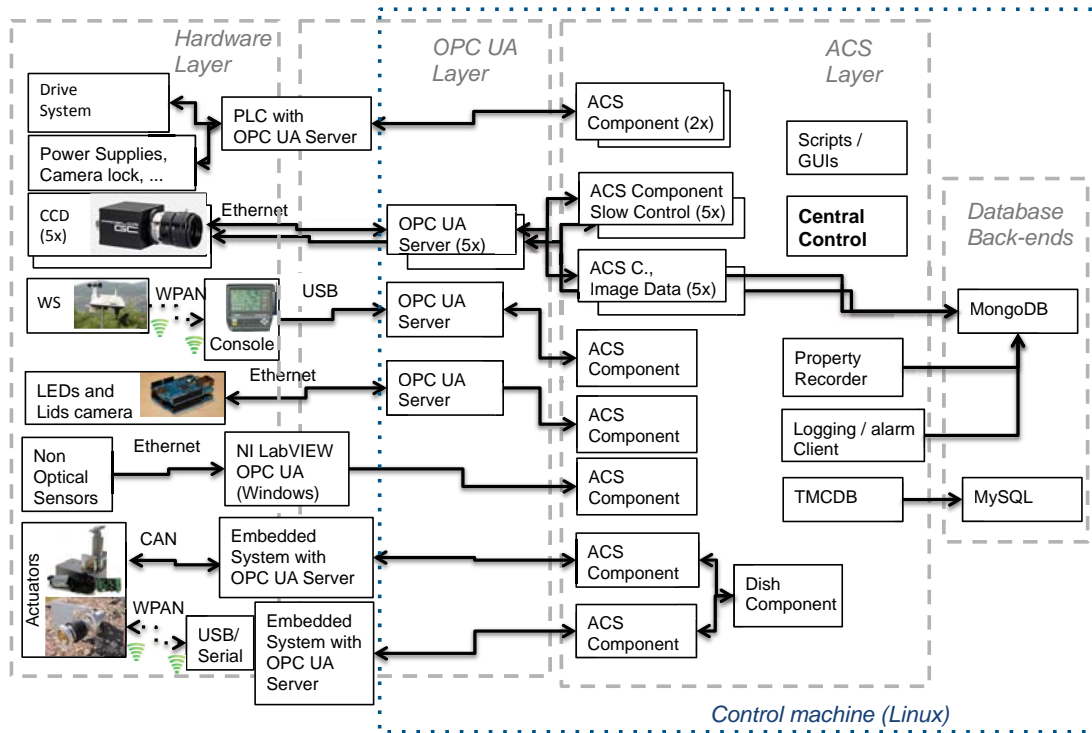
Figure 1. The MST prototype and instrumentation for control and readout. See text for details.
