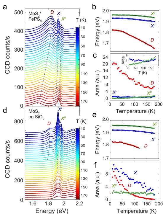
Figure 3. (a–c) Temperature evolution of photoluminescence within the range of 10–180 K in steps of 5 K in the heterostructure sample (a) PL spectra. (b) Peak energy positions extracted from a fit of the data to a multiplex model (see Supporting Information Section S13) as a function of temperature. The solid line represents the fit to a standard semiconductor model. (c) Peak areas. (d–f) Photoluminescence as a function of temperature in the control sample. (d) PL spectra. (e) Peak energy positions. (f) Peak areas.
