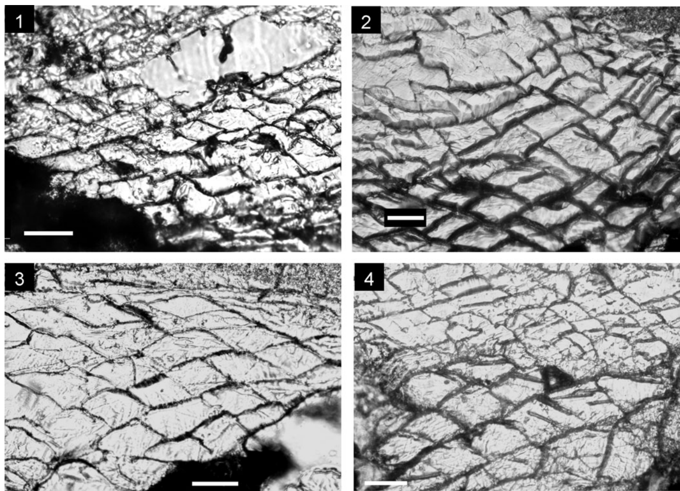
Figure 5. Eurinoid microstructure of the secondary layer of the shell in some wellerelloid taxa analyzed. (1) Cirpa planifrons (Ormós, 1937), section at 2.20 mm from the apex in the specimen CCA.8.Cpla.X. (2) Cirpa lucentina n. sp., section at 2.30 mm from the apex in the specimen I.12.T26(26).1. (3) Cirpa briseis (Gemellaro, 1874), section at 2.00 mm from the apex in the specimen CCB5.2. (4) Salgirella alberti (Oppel, 1861), section at 2.40 mm from the apex in the specimen I.12.T26(26).2. All scale bars represent 50 \mu m.
