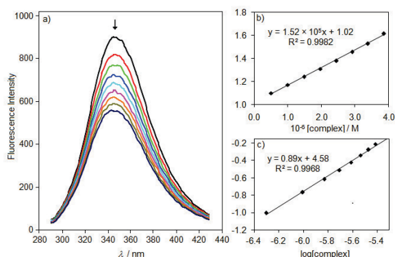
Figure 4. Interaction of 1b with BSA: a) spectrofluorimetric titration of BSA with complex; b) graphical determination of Stern-Volmer constant; c) graphical determination of binding constant and number of binding sites.
