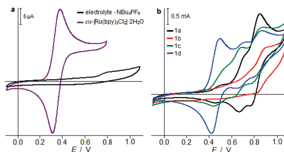
Figure 2. Cyclic voltammograms of a) cis -[Ru(bpy) 2 Cl 2 ]·2H 2 O and supporting electrolyte \text{NBu}_4\text{PF}_6 , b) 1a–1d , in acetonitrile solution; working electrode Pt wire vs Ag/AgCl reference electrode; scan rate 100 \text{ mV s}^{-1} ; E = 0.5 (E_{\text{pa}} + E_{\text{pc}}) ; \Delta E_{\text{p}} = E_{\text{pa}} - E_{\text{pc}} .
