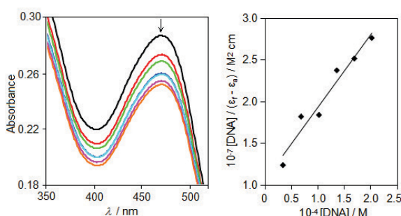
Figure 3. Spectroscopic titration of 1b ( 5 \cdot 10^{-5} M) with CT DNA ( 0 – 2 \cdot 10^{-4} M), A_{260} / A_{280} = 1.86 ) in 10 mM Tris-HCl buffer pH 7.42, T = 295 K, t = 2 min. Inset: Graphical determination of binding constant.
