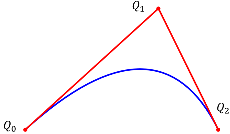
Figure 4.1: Notation of a polynomial quadratic curve.
