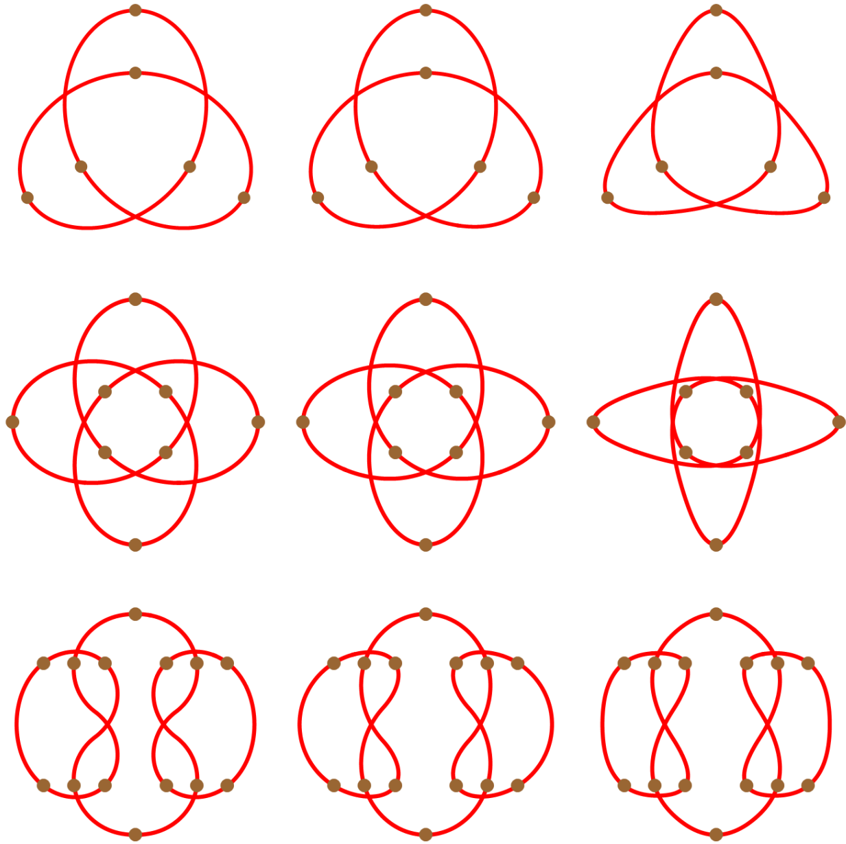
Figure 6.4: Comparisons between different weight choices. Left to right: min eccentricity weights, clamped min eccentricity weights, original \kappa -curve.
