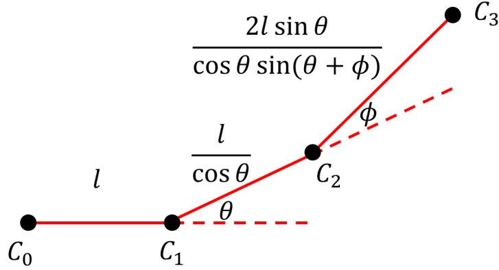
Figure 4.7: Our restricted cubic curve can be defined purely by the angles between three edges and the lengths of the edges according to the angles.
