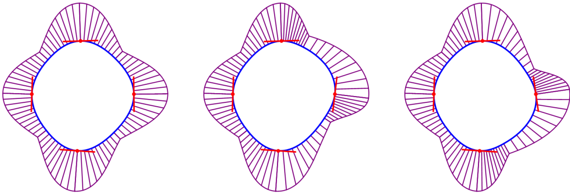
Figure 7.2: All the three pictures have the same input points and the same curvature assigned for each input point. Compare to the left picture, the tangent direction of the right point of the middle and the right pictures are rotated 7.5^\circ in the clockwise and counter-clockwise directions.
