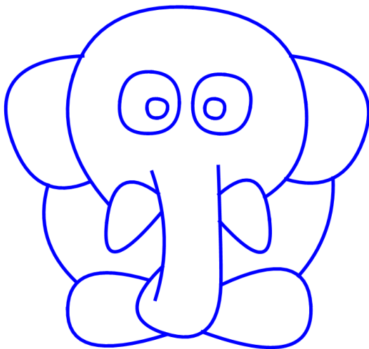
Figure 5.10: \kappa -Curve examples of a cartoon bear and elephant.
