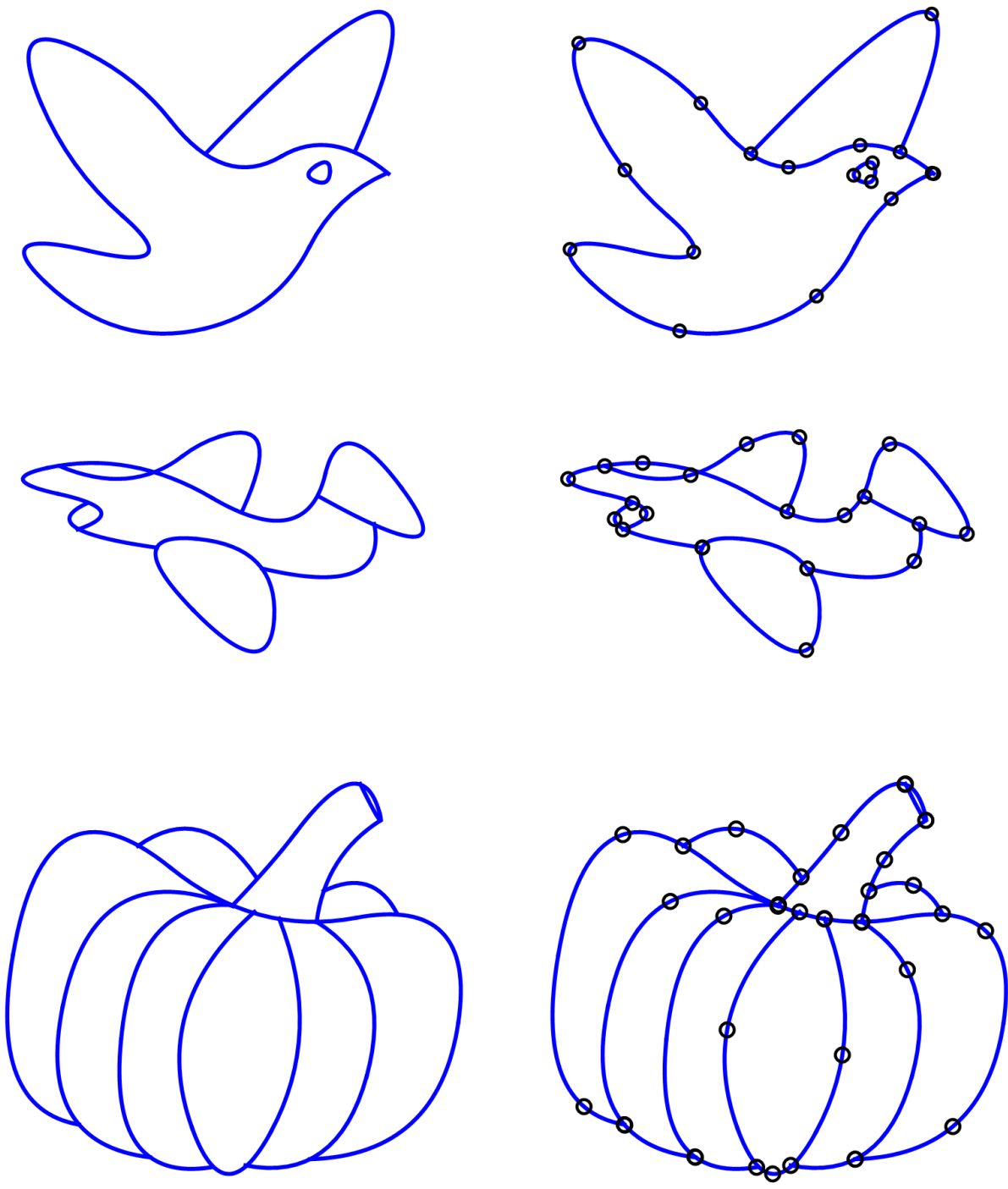
Figure 5.11: \kappa -Curve examples of a bird, a plane and pumpkin.
