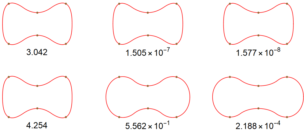
Figure 6.9: Curve optimization. Each image has the same input points with the error shown below. Each row shows the initial guess (left), after 60 iterations of refining the initial guess (middle), and the result of our optimization (right). The first row uses weight 1 while the second row are our clamped min eccentricity weights. The top middle picture corresponds to the \kappa -curve result in [4].
