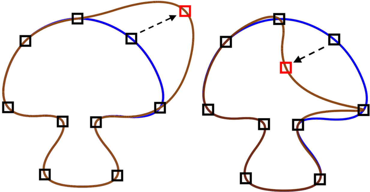
Figure 5.9: The original curve in blue with the new curve in brown drawn on top. While control points have a global influence on the curve, that influence drops dramatically with distance from the control point, which creates the effect of local influence.
