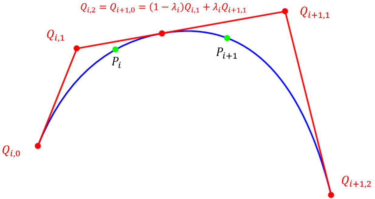
Figure 5.3: Connecting two polynomial quadratic curve segments.
