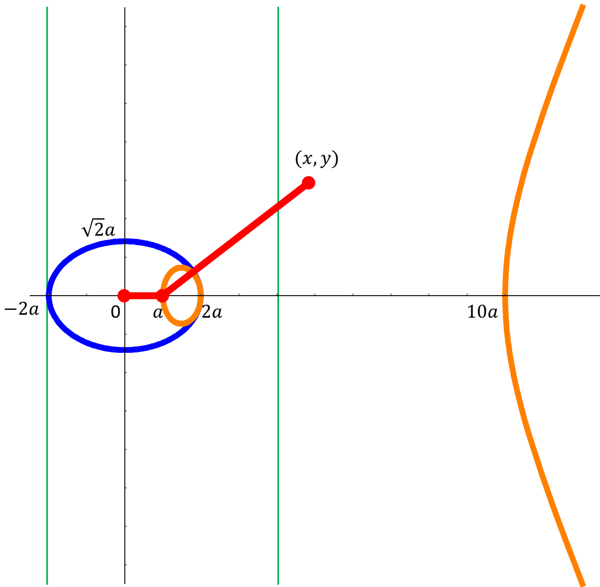
Figure 4.6: The regions of different monotonicity of our cubic curve.
