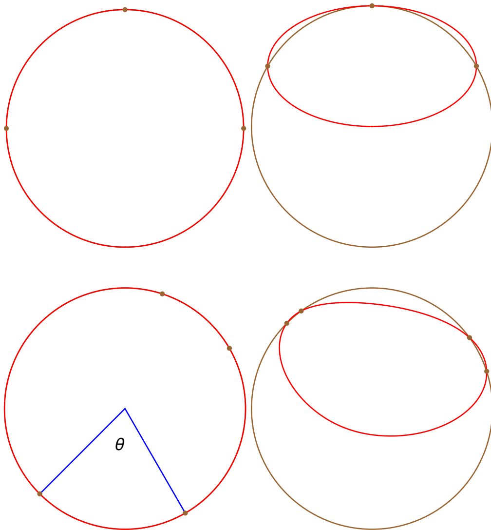
Figure 6.10: Circle reproduction with three (top) or four points (bottom). The left column has input points with central angles less than \pi . The right has points with one central angle over \pi , which leads to a non-circular curve.
