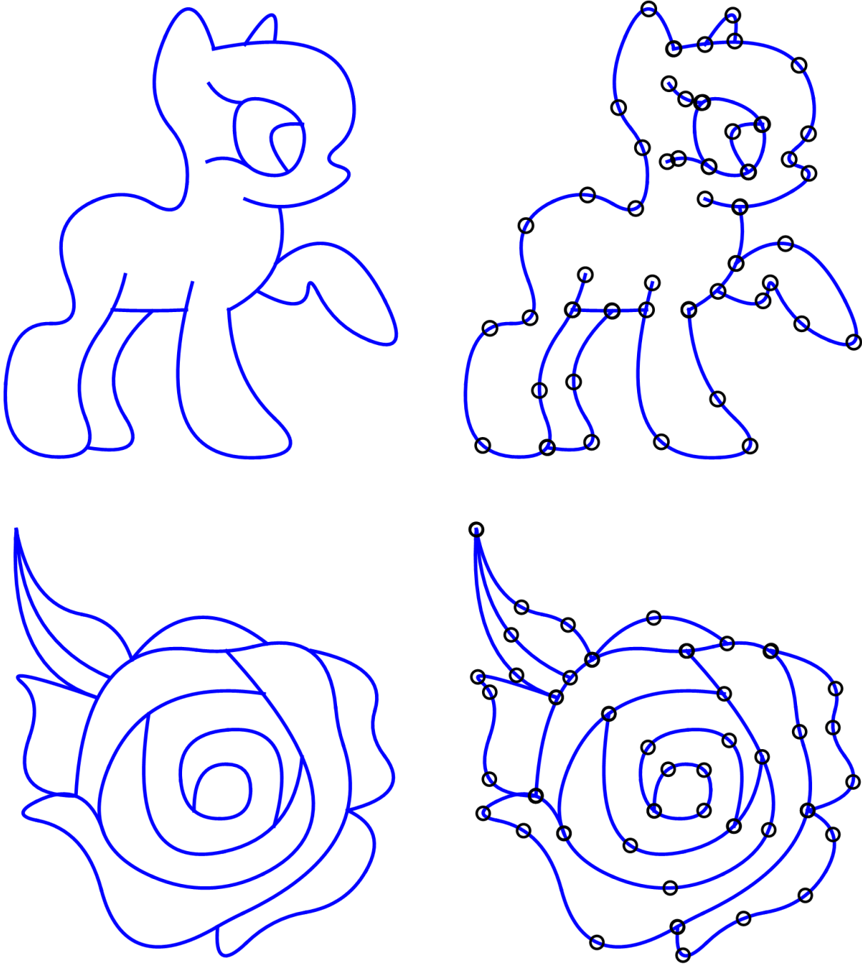
Figure 5.12: \kappa -Curve examples of a horse and a rose.
