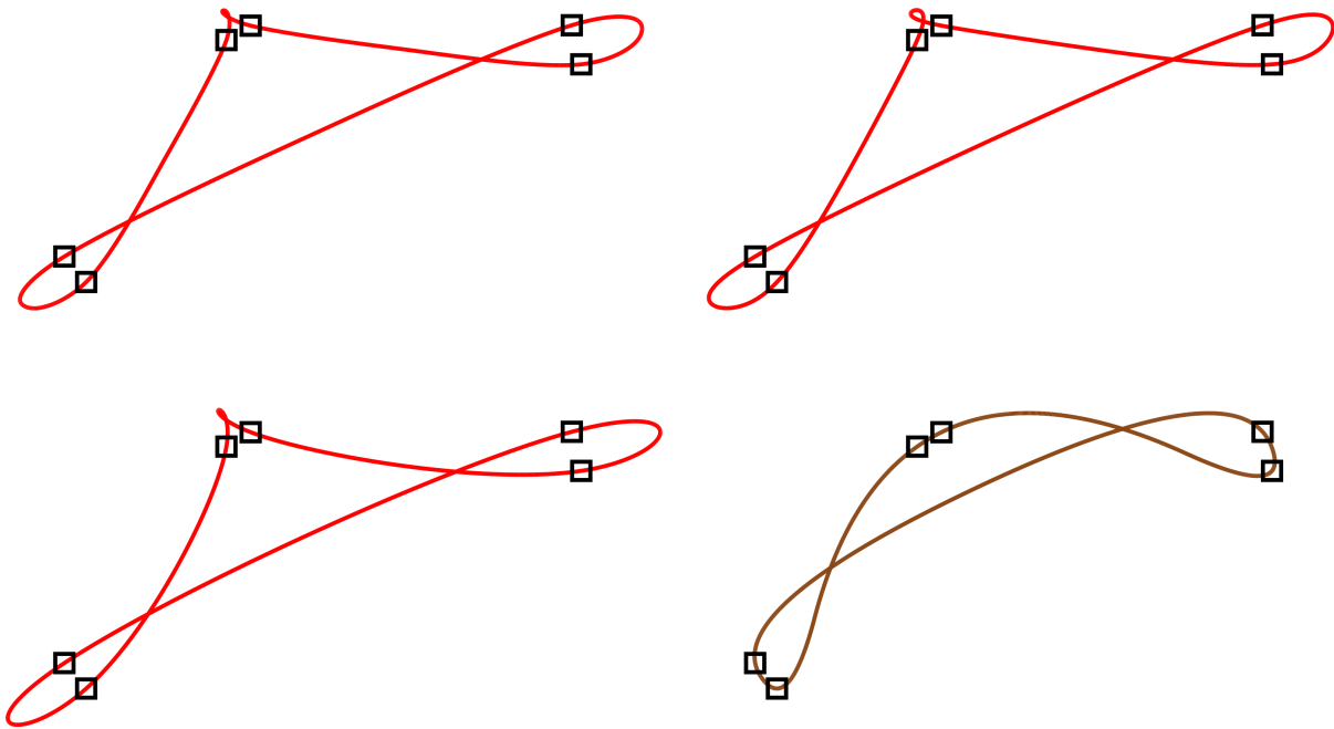
Figure 1.2: Comparison of different C^2 curves with the same control points. First row from left to right: 6-point interpolatory subdivision curve [1], C^2 Catmull-Rom spline [2]; second row from left to right: C^2 interpolating cubic B-spline [3], \kappa -Curve[4].
