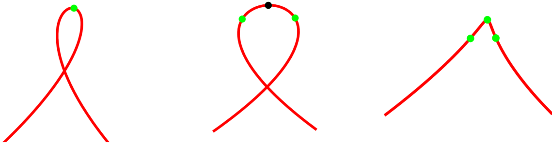
Figure 4.4: Examples of cubic curves with different critical points. The left and right picture have one and three local maximum curvature points in green. The middle one has two local maximum curvature points in green and one local minimum curvature point in black.
