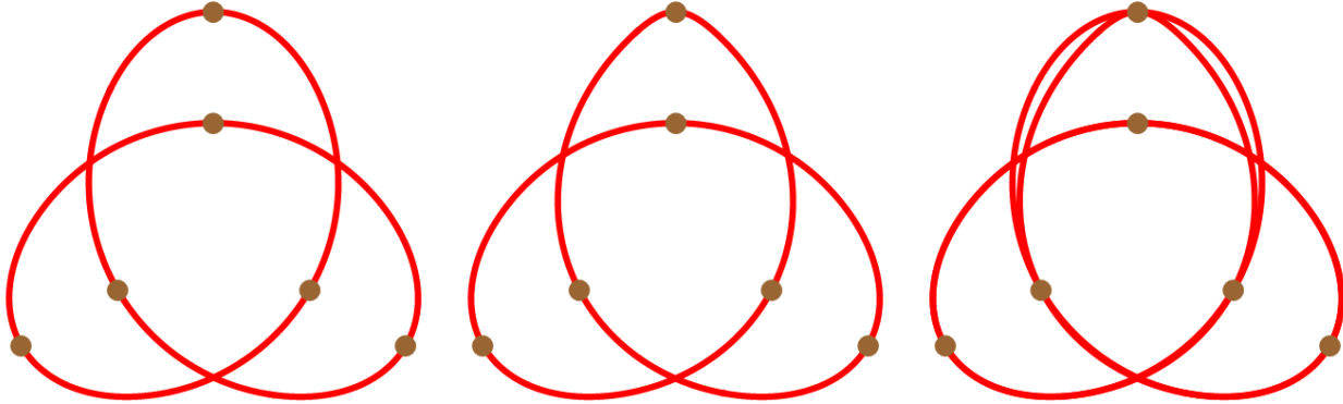
Figure 6.6: Clamped minimum eccentricity weight curves with tension values \mu_i set to 1 (left) and with the weight of the top input point set to 2 (middle). The right picture shows the overlapping curves for comparison.
