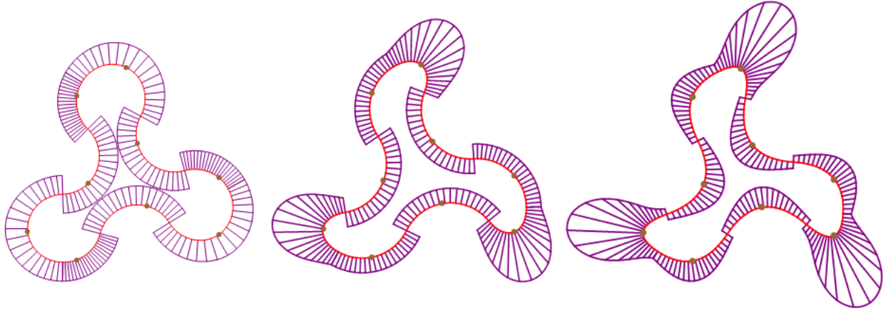
Figure 6.3: The purple lines show curvature normals. Each picture uses the same input points with different weight functions. From left to right: min-eccentricity weights, clamped min-eccentricity weights, and the original \kappa -curve.
