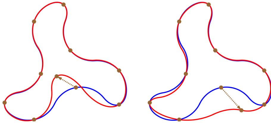
Figure 6.8: The blue/red curves show our curves before/after moving a single input point. Despite the global nature of the optimization, the change in the curve tends to decrease with distance from the input point.
