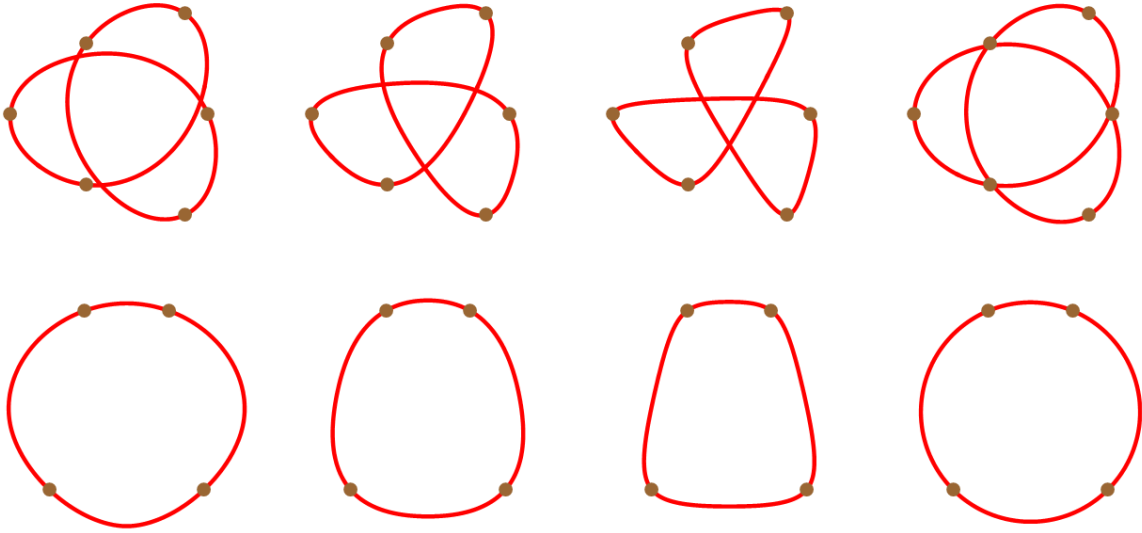
Figure 6.2: Each row contains the same input points \{P_i\} but uses different weights for the input points in each column. The weights from left to right are: 0.6, 1, 2, and our clamped min eccentricity weight.
