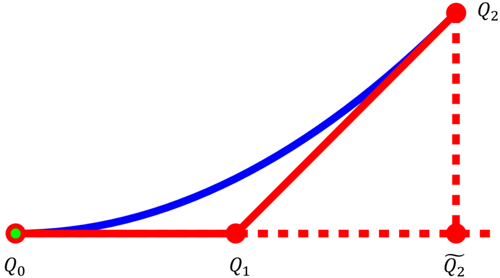
Figure 4.2: Geometric condition of a quadratic curve with monotonic curvature. |Q_0Q_1| = |Q_1\tilde{Q}_2| and the green spot is the critical point of the parabola.
