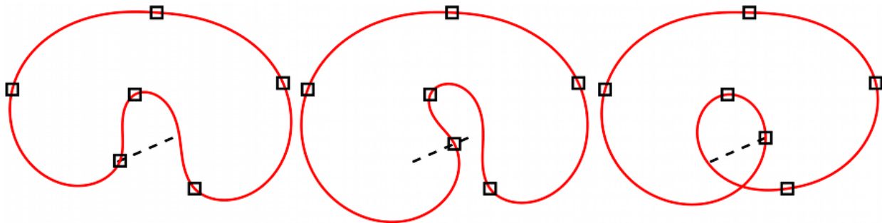
Figure 3.1: Moving one control point continuously for a piecewise clothoid curve can result in a discontinuous change in the curve as shown on the right where the curve suddenly flips over.
