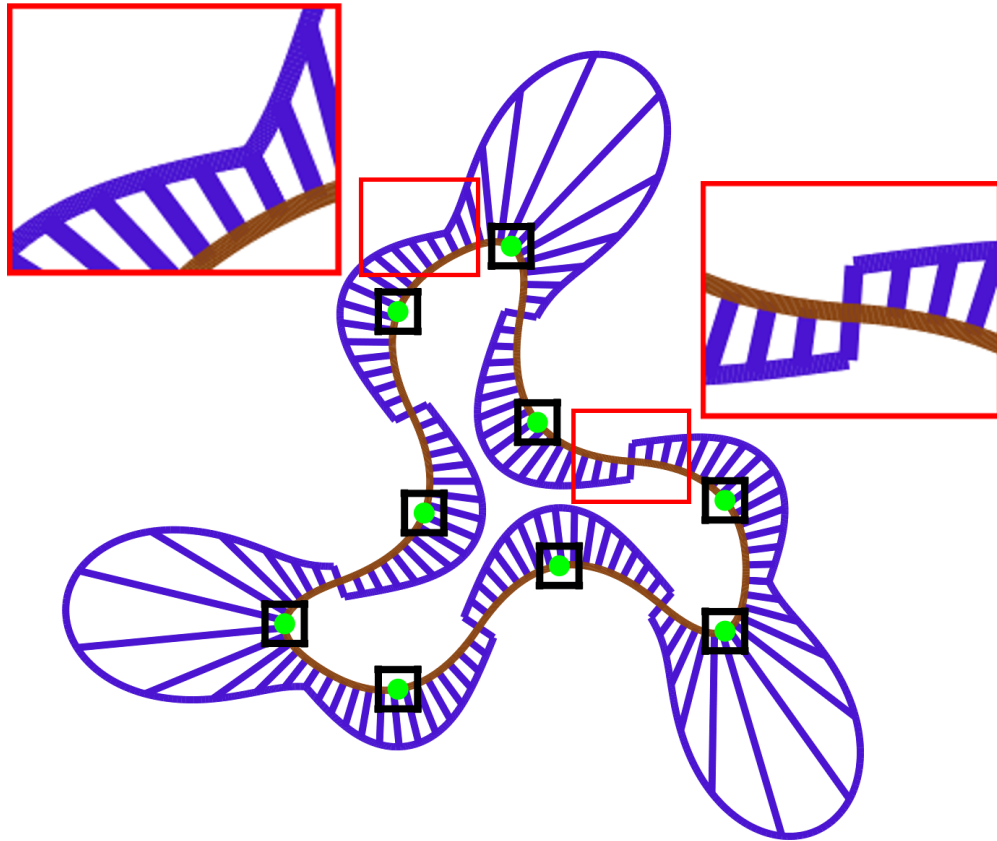
Figure 5.6: Our curve (brown) shown with control points as block boxes. Green points are positions of local maximal curvature magnitude. We also draw the curvature normal for the curve (purple). Our curve is G^2 everywhere as shown in the highlighted region except at inflection points where the curve is G^1 and the sign, but not magnitude, of the curvature changes.
