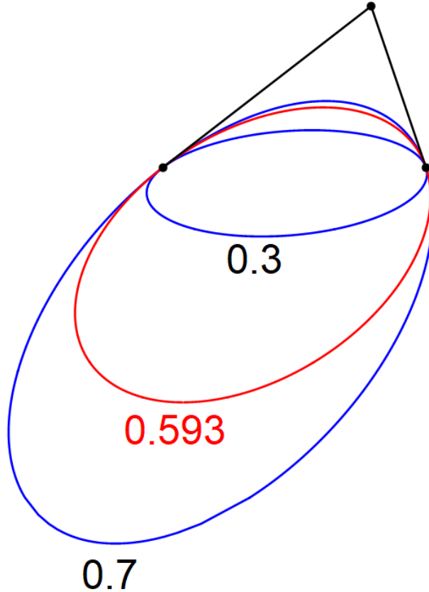
Figure 6.1: A rational Bézier curve with unit weights for the two end-points and different ellipses generated by modifying the weight of the central control point, which is set to 0.3 (blue), 0.7 (blue), and 0.593 (red), which is the minimal eccentricity weight for these control points.
