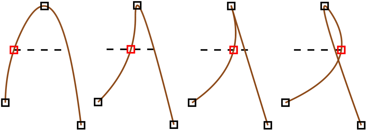
Figure 5.8: The creation of a cusp, which can only happen at control points with our method.
