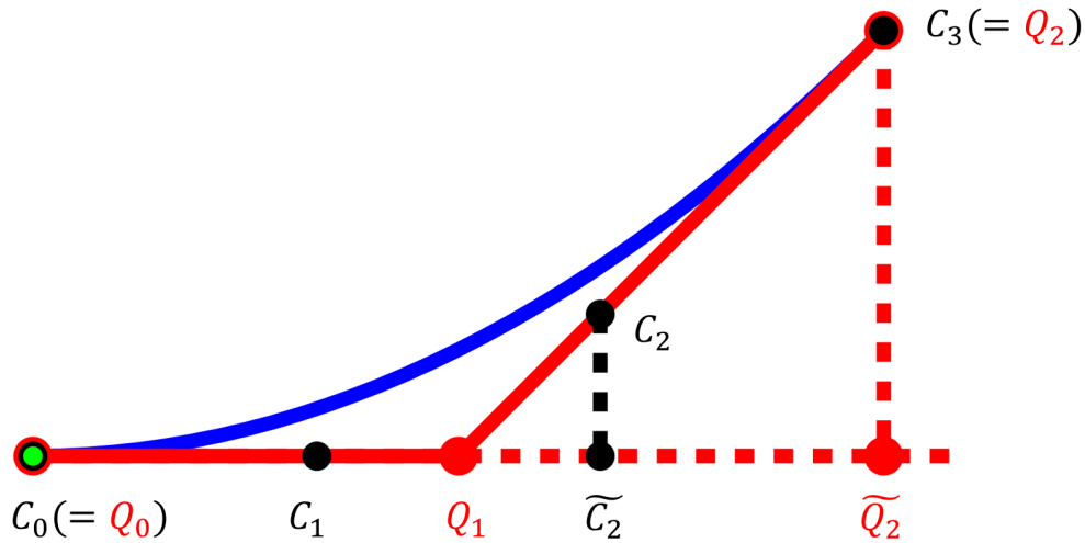
Figure 4.5: Elevation to cubic curve from a quadratic curve. In this picture, Q_1 is the middle point of line segment Q_0\tilde{Q}_2 so that Q_0 is the critical vertex of the parabolas. The red points and lines are the quadratic control polygon. The black points are cubic control points. The green spot is local maximum curvature of the blue curve.
