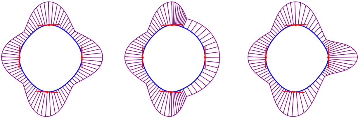
Figure 7.3: The three pictures have the same input points and all input points are assigned the same tangent directions. Compared to the left picture, the curvature of the right point in the middle and the right pictures are multiplied by 0.7 and 1.4.
