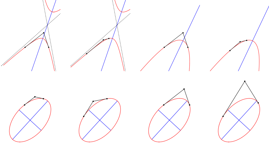
Figure 4.3: All eight cases of critical points a rational quadratic curve segment can have. Rational Bézier curves may have 0, 1 or 2 critical points of curvature within the parameter range (0,1) . Solid black lines are Bézier control polygons, red lines are rational Bézier curves, blue lines are axes of symmetry for the conic sections. The first row shows a hyperbola (first two images) and a parabola (last two images), each of which can have one or zero max curvature points within a rational Bézier curve. The last row shows an ellipse, which may have 0, 1 min, 1 max, or 1 min and 1 max curvature points.
