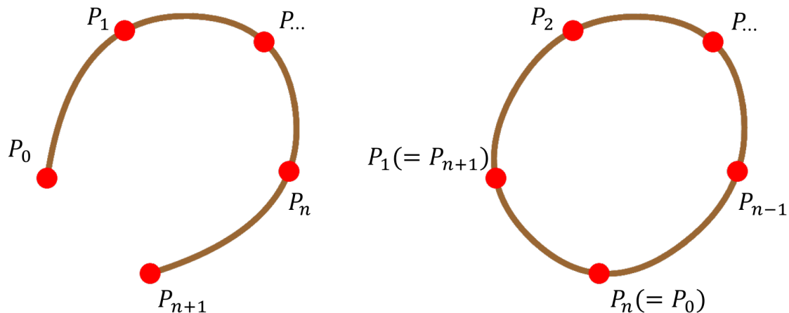
Figure 5.1: Notation and subscripts of the input points for open and closed curves.
