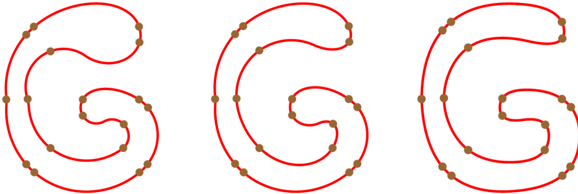
Figure 6.5: An asymmetric example with non-uniformly spaced control points. From left to right: min eccentricity weights, clamped min eccentricity weights, original \kappa -curve.
