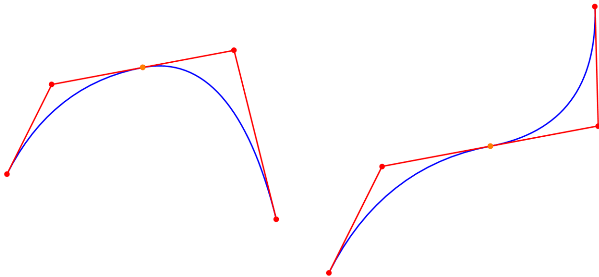
Figure 5.2: Two quadratic curve segments can be connected in a convex or a concave way satisfying G^1 condition.
