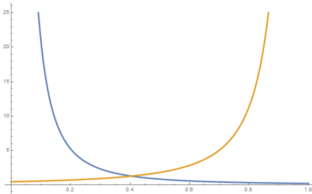
Figure 5.4: Plot of the curvature on the two sides of the join point when moving from one end to the other end on the line segment.
