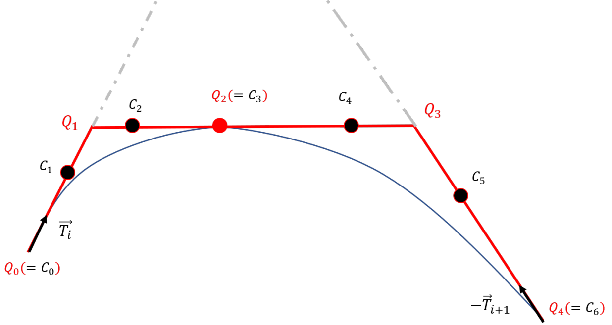
Figure 7.1: Connect two single quadratic or cubic pieces as a whole curve segments. Quadratic control points are rendered in red \{Q_i\} , while the cubic control points \{C_i\} are in black.
