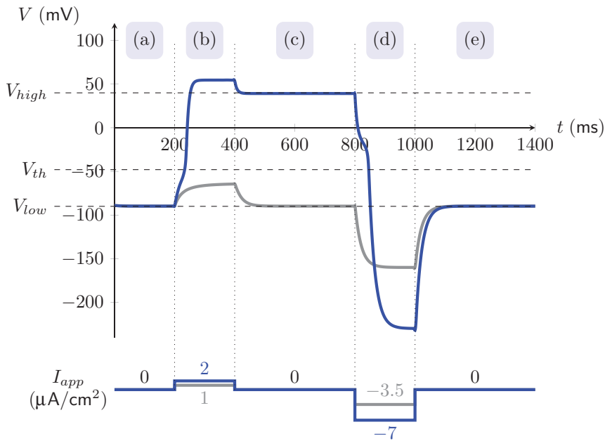
Figure 11.4 Bistability of the I_{Cav} + I_L membrane model (Eq. 11.1) observed in response to pulses of applied current ( I_{app} ).
