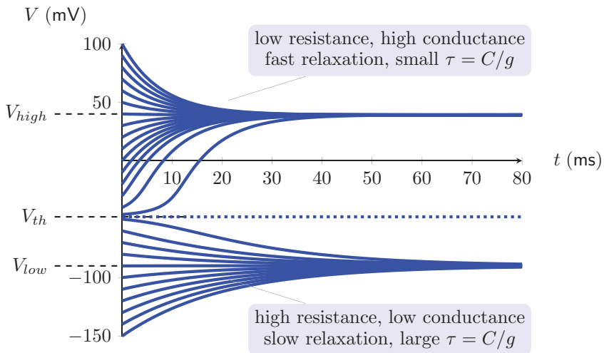
Figure 11.2 The phase diagram for a membrane that expresses I_{CaV} and I_L in the absence of applied current ( I_{app} = 0 ). Question: When V \approx V_{low} (or V_{high} ), the dynamics are well approximated by exponential relaxation. For which steady state is the exponential time constant larger (slower relaxation)?
