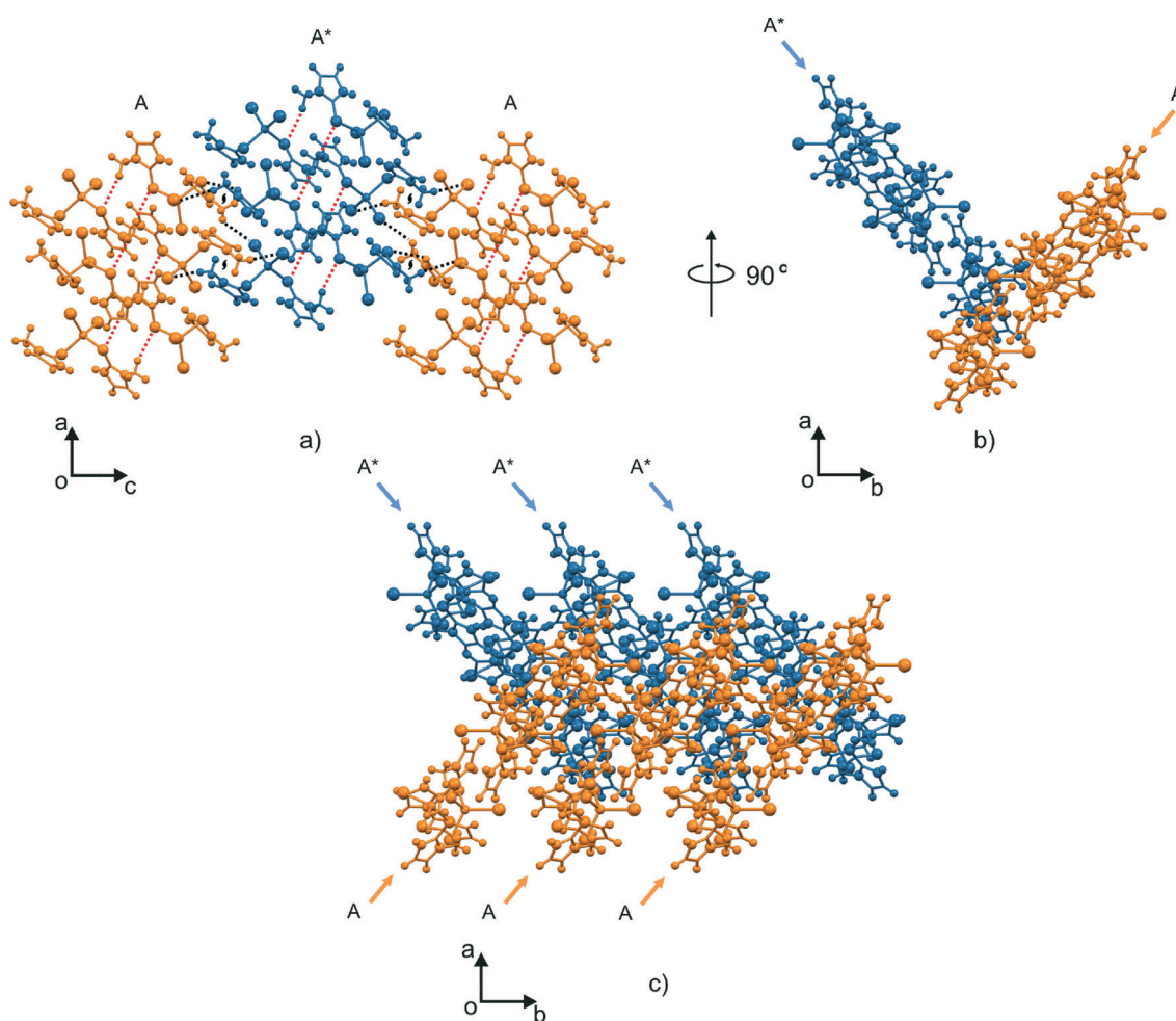
Fig. 5 Representation of the crystal packing of the complex [Zn(MelmSH)_2]_2 . a) Crystal packing viewed along the [010] direction ( 2_1 screw axes are indicated in black). Intermolecular interactions connecting adjacent chains are indicated by black dashed lines. Red colour is used for interactions within the molecular arrangements A; b) development of the 1-D chains A along the [001] direction under the effect of n -glide symmetry; c) crystal packing viewed along the [001] direction. The molecules are colour coded depending on the direction of propagation of the 1D chains: orange as the [110] direction, blue as the [1\bar{1}0] direction. The differences in the orientation of the chains are also indicated by using different labels (A and A*) and coloured arrows.
