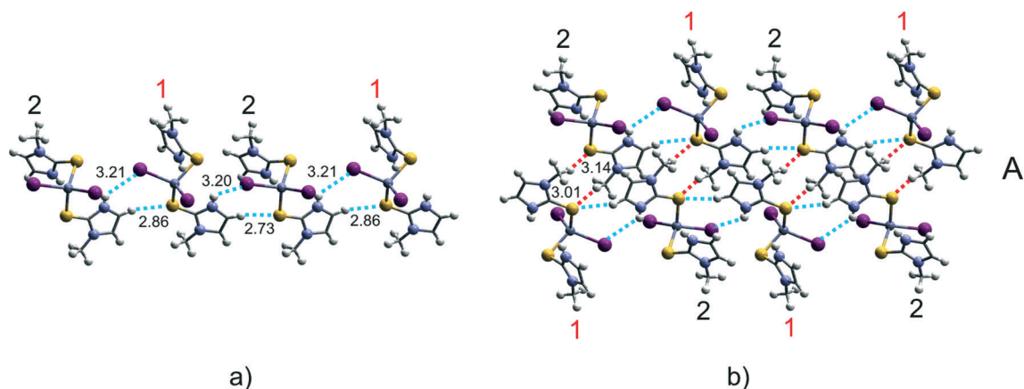
Fig. 4 Representation of the main molecular arrangements identified for the structure of the complex [Zn(MelmSH)_2]_2 . a) Single 1-D chain, built by intermolecular interactions involving the two independent molecules 1 and 2; b) molecular arrangement A. The molecular arrangements are oriented to better show the intermolecular interactions. Bond distances are in Å.
