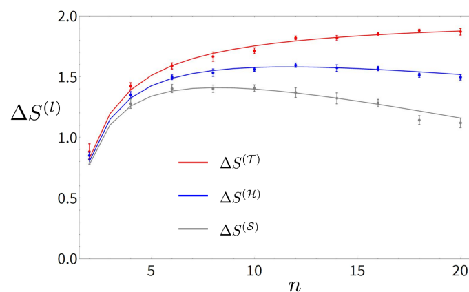
Fig. 2. CHSH inequality violation in the spatial and temporal domain. Classical bound violation \Delta S^{(l)}(n) = S^{(l)}(2n) - (2n - 2) ( l = \mathcal{T}, \mathcal{H}, \mathcal{S} ) for the multiparameter CHSH inequalities in the temporal (red), spatial (gray), and hybrid (blue) domains. The dots represent the experimental results, with the uncertainty bars evaluated as statistical fluctuations among repeated measurement sets, while the solid curves show the theoretically expected values (for the correlations belonging to the spatial domain, deviations from the ideal case due to the V_S = 0.982 estimated visibility of the generated |\psi_{-}\rangle state were considered).
