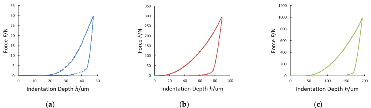
Figure 8. Loading–unloading curves of the HV tests on aluminum alloy: (a) HV3; (b) HV30; (c) HV100.
