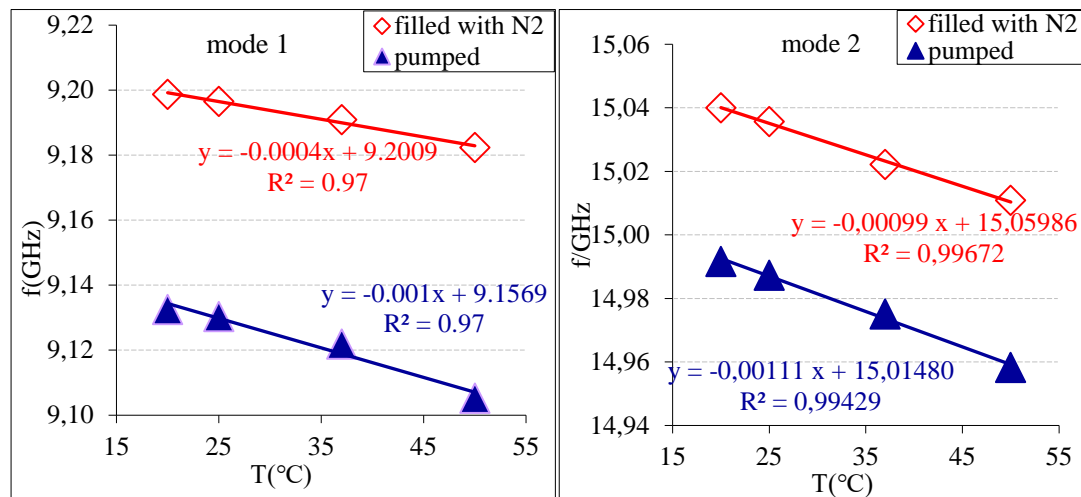
Figure 7. Frequency-temperature sensitivity for mode 1 and 2 with cavity pumped and filled with nitrogen respectively
